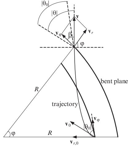
Fig. 1. – The geometrical scheme of proton motion.
