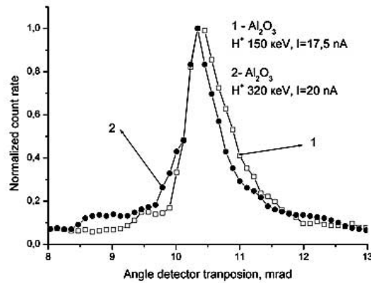
Fig. 9. – Angular distribution of H + ions transmitted through capillaries in the Al 2 O 3 membrane without metallic coverage at 0° tilt angle: 1–150 keV, I = 17.5 nA; 2–320 keV, I = 20 nA.
