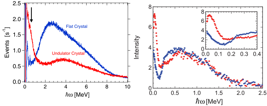
Fig. 4. – (Colour on-line) Left panel: raw photon spectra at (110) planar channeling of 855 MeV electrons for the flat (blue) and the undulator crystal (red) with effective thicknesses of 49.5 \mu\text{m} and 39.6 \mu\text{m} , respectively. Data were taken with the NaI detector, see fig. 2. Right panel: deconvoluted photon spectra at (110) planar channeling of 270 MeV electrons for the flat (blue) and the undulator crystal (red). Data were taken with the Ge(i) detector shown in the inset of fig. 2.
