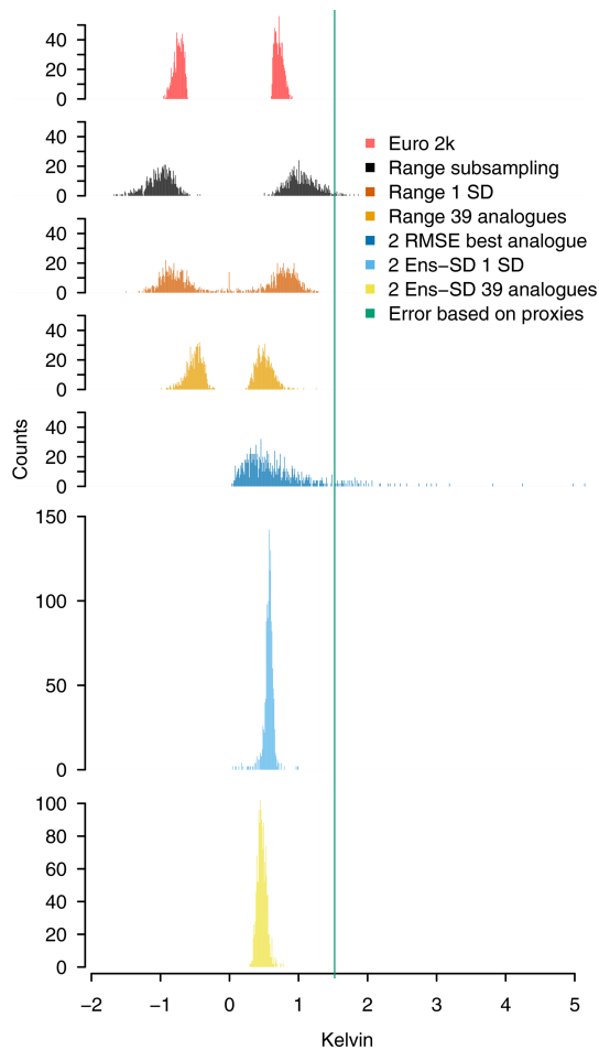
Figure 12. Comparison of uncertainty estimates: from top to bottom, histograms in bins of 0.01 K for Euro 2k 2 standard deviation uncertainty (red), range of subsampling ensemble (black), range of fixed 1 noise standard deviation ensemble (dark orange), range of 39 analogues (light orange), assumed 2 standard deviation interval for the MSE-based uncertainty estimate for the single best analogue (dark blue), ensemble-variance-based 2 standard deviation interval for the 1 noise standard deviation (light blue), ensemble-variance-based 2 standard deviation intervals for the 39 analogues (yellow). We only show one-sided estimates when the estimates are symmetric. The green line throughout the panel marks the uncertainty estimate based on the proxy noise.
