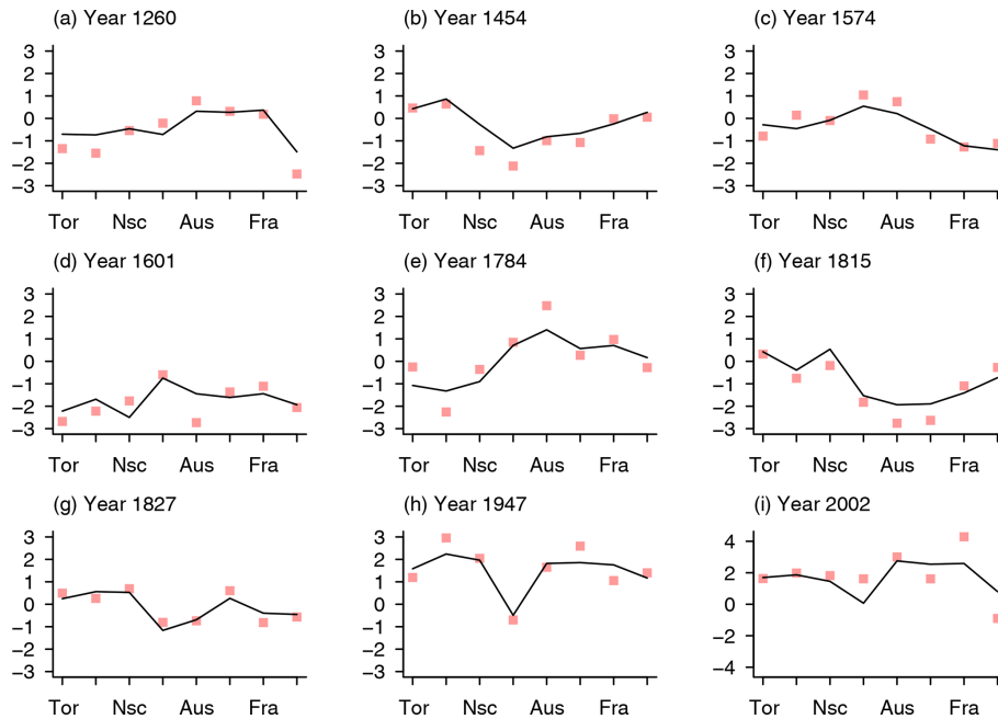
Figure 4. Normalized proxy values (squares) for proxies included and the values of the best analogue for selected years (lines). Proxy locations on the x axes are from PAGES 2k Consortium (2013a): Tor (Torneträsk, Sweden), Jae (Jämtland, Sweden), Nsc (northern Scandinavia), Car (Carpathians, Romania), Aus (Alps, Austria), Swi (Alps, Switzerland), Fra (Alps, France), Pyr (Pyrenees, Spain).
