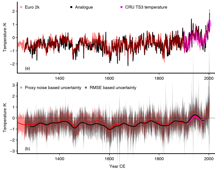
Figure A1. The best-analogue reconstruction as in Fig. 2 but relative to the observational period (1901–2003 CE). (a) The interannual temperature reconstruction is in black, the red line is the area mean Euro 2k reconstruction, magenta is the observational CRU temperature adjusted to the mean of the reconstruction over its time range. The analogue reconstruction is rescaled by the variability from one of the simulations. Panel (b) is the same as (a) but for 47-point Hamming filtered data; we further add the uncertainty estimates for the interannual data: red is the unsmoothed Euro 2k uncertainty, the lighter grey envelope is a 2 standard deviation uncertainty based on the correlation between the proxies and the observations at the proxy locations, the darker grey envelope is a 2 standard deviation uncertainty based on a MSE estimate. Panel (b) adds a zero line as visual assistance.
