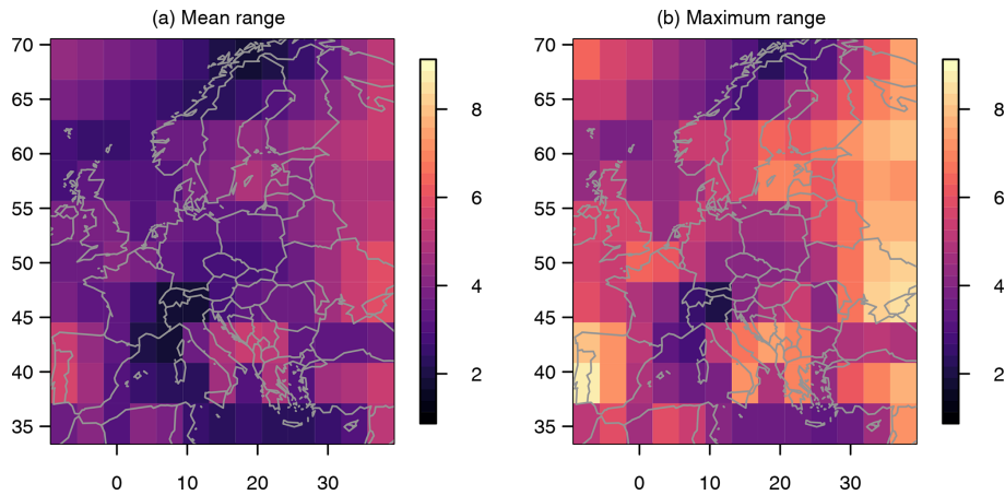
Figure 10. The local range of analogues over the reconstruction period: (a) mean range; (b) maximum range occurring over the period.
