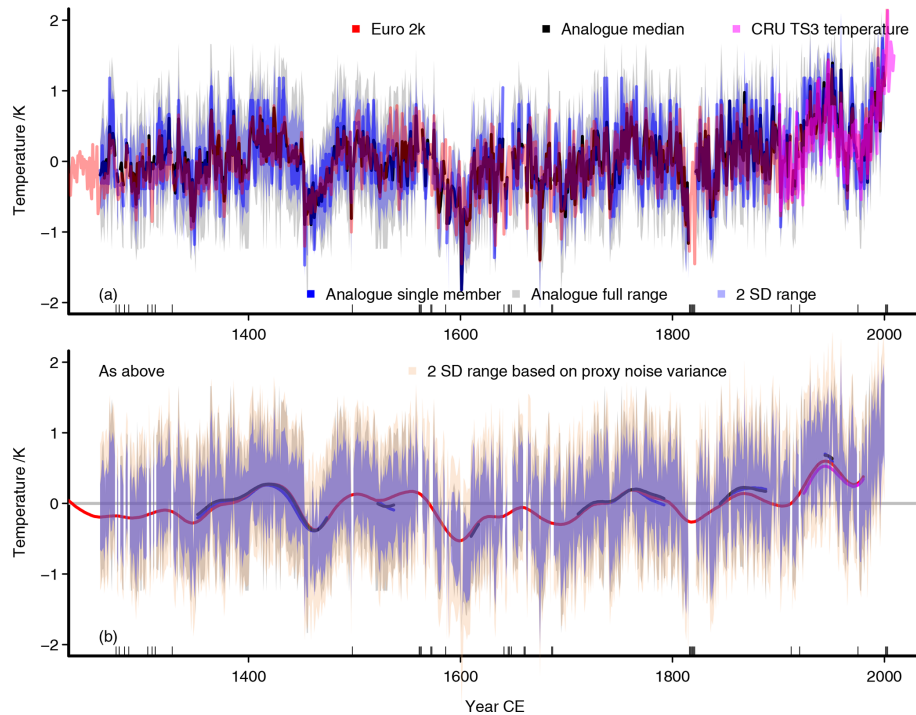
Figure 8. Analogue reconstruction based on an 1\text{ SD}_{\text{noi}} uncertainty of the proxies. (a) Interannual data: red, the Euro 2k reconstruction; black, the analogue median; blue line, a single analogue member; blue shading, 2 standard deviation uncertainty range around the analogue median based on variability of the analogues; grey shading, the full range of analogues; marks at horizontal axis mark unsuccessful analogue searches. Panel (b) is the same as (a) for 47-point Hamming filtered data, but we add a 2 standard deviation uncertainty based on the square root of the proxy noise variances in brown, as also shown in Fig. 2. Panel (b) adds a zero line as visual assistance.
