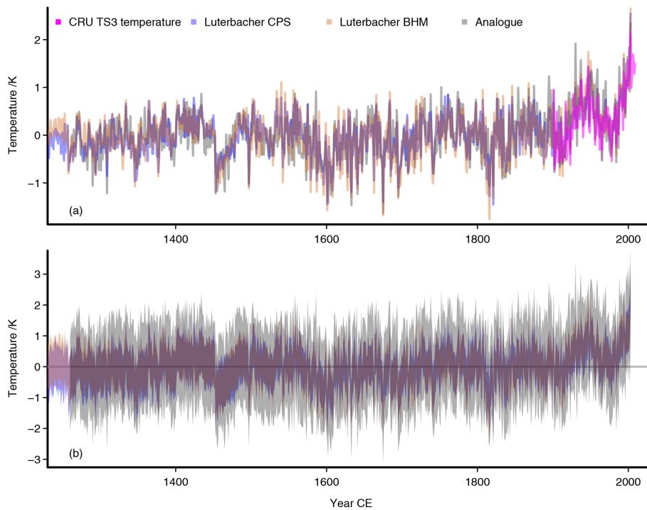
Figure A3. Comparison of the reconstructions of Luterbacher et al. (2016) to the best-analogue reconstruction (see also Fig. 2): (a) the inter-annual single best-analogue temperature reconstruction in grey, the blue is the composite-plus-scaling (CPS) reconstruction of Luterbacher et al. (2016), and the brown line is the area mean of their Bayesian hierarchical modeling reconstruction; magenta is the observational CRU temperature adjusted to the mean of the analogue reconstruction over its time range. The analogue reconstruction is rescaled by the variability from one of the simulations. Panel (b) is the same as (a) but for the 95 % uncertainties of the reconstructed datasets. Differences between the Luterbacher CPS and the Euro 2k mean reconstructions are smaller than 0.005 K. Panel (b) adds a zero line as visual assistance.
