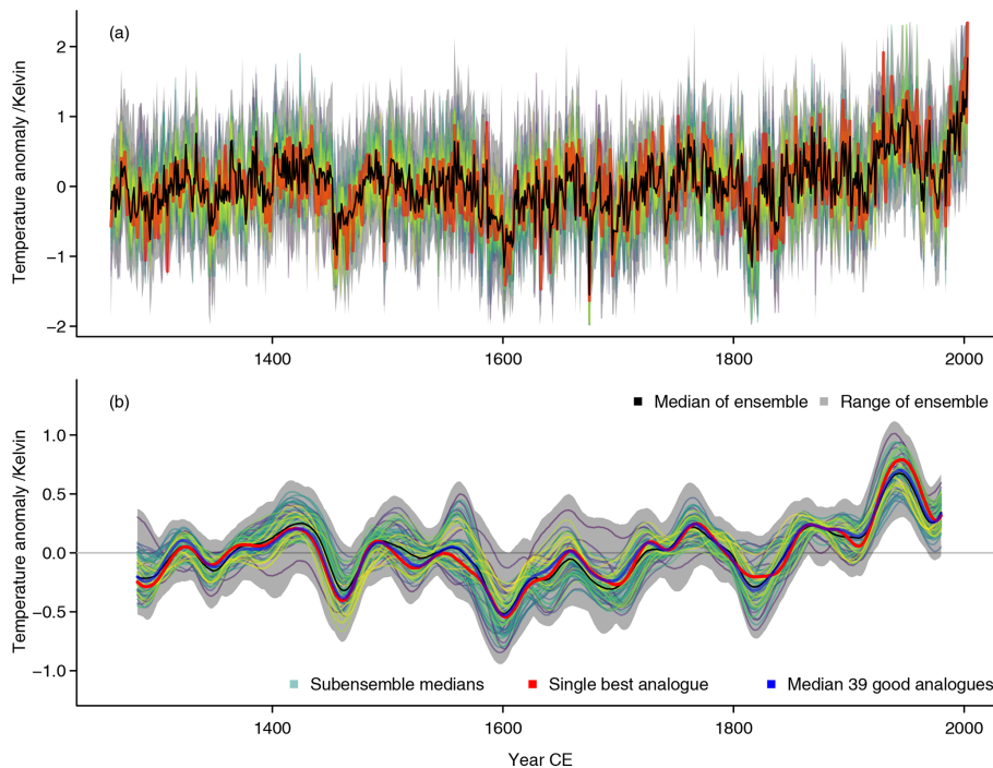
Figure 11. Ensemble of subsampled reconstructions. (a) Interannual data, (b) data smoothed with 47-point Hamming filter. Both panels show in grey the full range of 6500 reconstructions based on four proxies and only half of the simulated fields, in black the median of all 6500 reconstructions, and in red the single best-analogue reconstruction based on the full data. Further colored lines are medians of the 65 sub-ensembles using different sets of four proxies. Panel (b) adds a zero line as visual assistance and additionally shows the median of the 39 good-analogue reconstructions.
