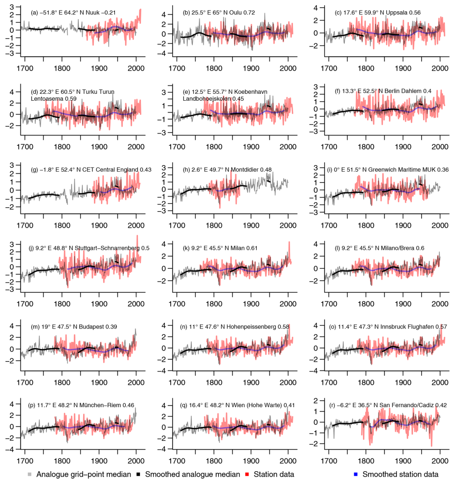
Figure 13. Comparison of local grid-point analogue data for the fixed 1 standard deviation approach with an arbitrary selection of regionally representative data from BEST. Location, station name, and correlation over available station data are at the top of the panels. Grey and black indicate the interannual and smoothed analogue medians. Red and blue lines are the interannual station data and their smoothed estimate. The x axes are years CE. The y axes are temperature anomalies in Kelvin relative to the period where both datasets are available.
