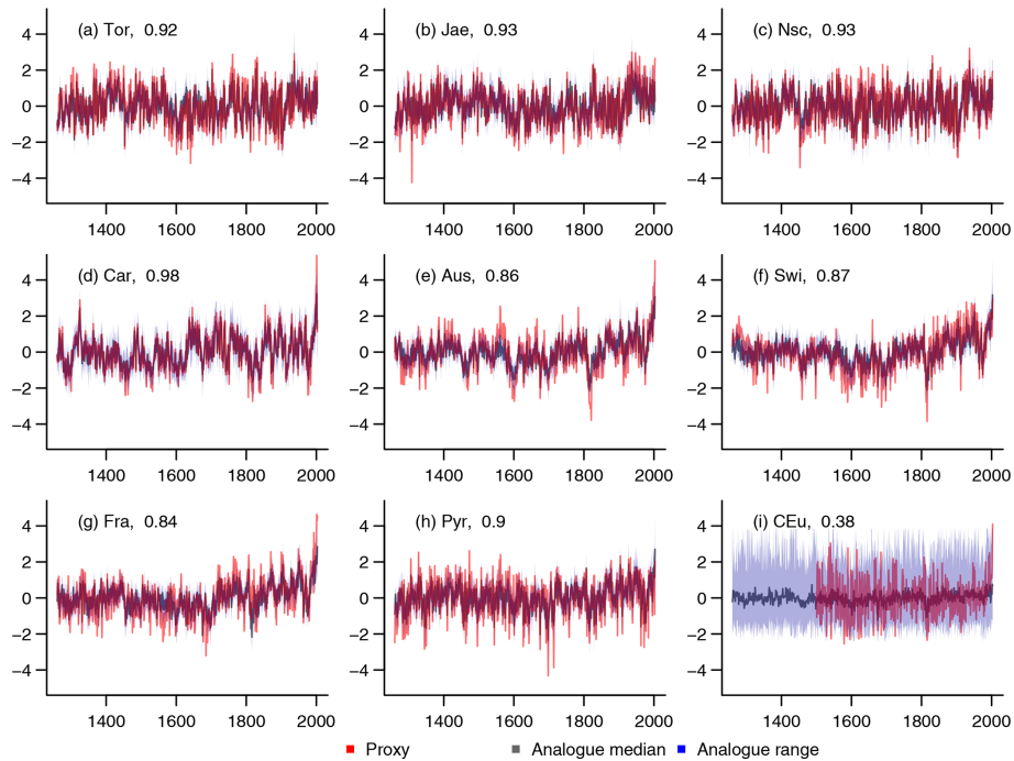
Figure 6. Analogue reconstruction values at the locations of the included proxies. Shown are the normalized proxies in red, the median of 39 analogue values in black, and the full range of the 39 local analogues in blue. The x axes are years CE. Correlations between the local reconstruction median and the proxy series are given as numbers next to the proxy IDs in each panel.
