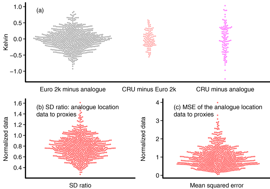
Figure 3. Further information about the single best-analogue reconstruction: (a) swarm plots for the differences between different datasets relative to their periods of overlap: grey is the Euro 2k reconstruction minus the single best analogue, red is the CRU TS data minus the Euro 2k reconstruction, and magenta is the CRU TS data minus the single best analogue. Since the data are relative to their overlapping period, the visualization hides potential biases. (b) Ratio between the standard deviations of the normalized analogue values at the closest grid points to the normalized proxy values. (c) Mean squared error between the normalized analogue grid-point values and the normalized proxies, i.e., the basis for one of the uncertainty estimates in Fig. 2. Swarm plots are categorical scatter plots that ensure that points do not overlap.
