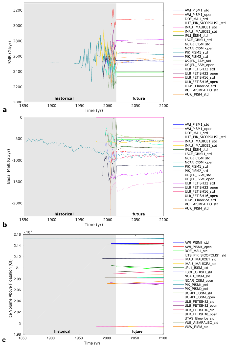
Figure 1. Evolution of surface mass balance (a, in Gt/yr), basal melt rate (b, in Gt/yr), and volume above floatation (c, in Gt) during the historical and ctrl_proj experiments for all the simulations performed with the open and standard framework.
