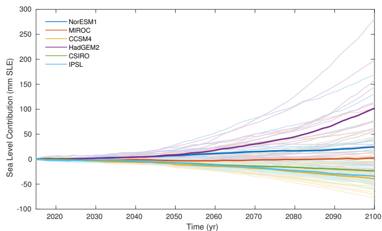
Figure 7. Evolution of ice volume above floatation (in mm SLE) over 2015–2100 period with medium forcing from the six CMIP5 AOGCMs and RCP 8.5 scenario relative to ctrl_proj. Thin lines show results from individual ice sheet model simulations, and thick lines show mean values averaged for each AOGCM.
