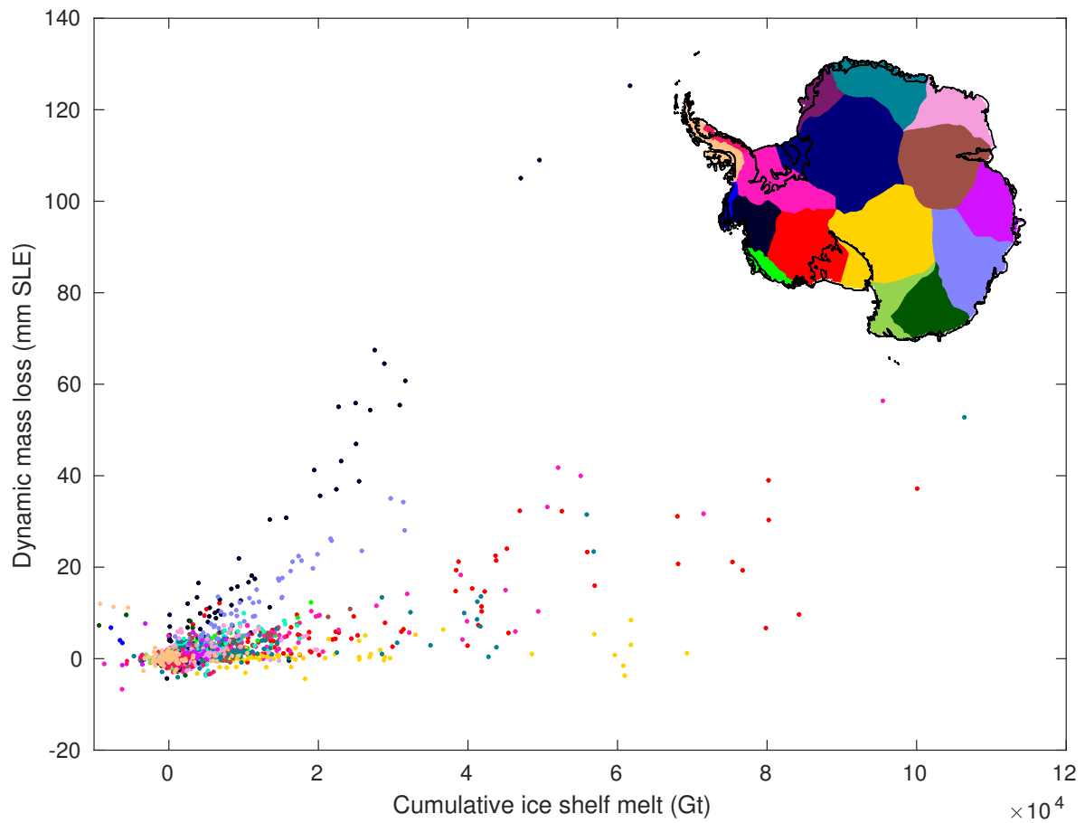
Figure 15. Dynamic mass loss over the 2015-2100 period as a function of cumulative ocean induced basal melt over the same period for the 18 main Antarctic basins (Rignot et al., 2019) for all RCP 8.5 experiments. Antarctic map shows the location of the 18 basins.
