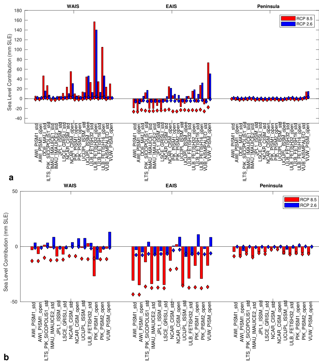
Figure 10. Regional change in volume above floatation (in mm SLE) and integrated SMB changes (diamond shapes, in mm SLE) for 2015–2100 under RCP 8.5 (red) and RCP 2.6 (blue) scenario forcing from NorESM1-M (a) and IPSL (b) relative to ctrl_proj from individual model simulations.
