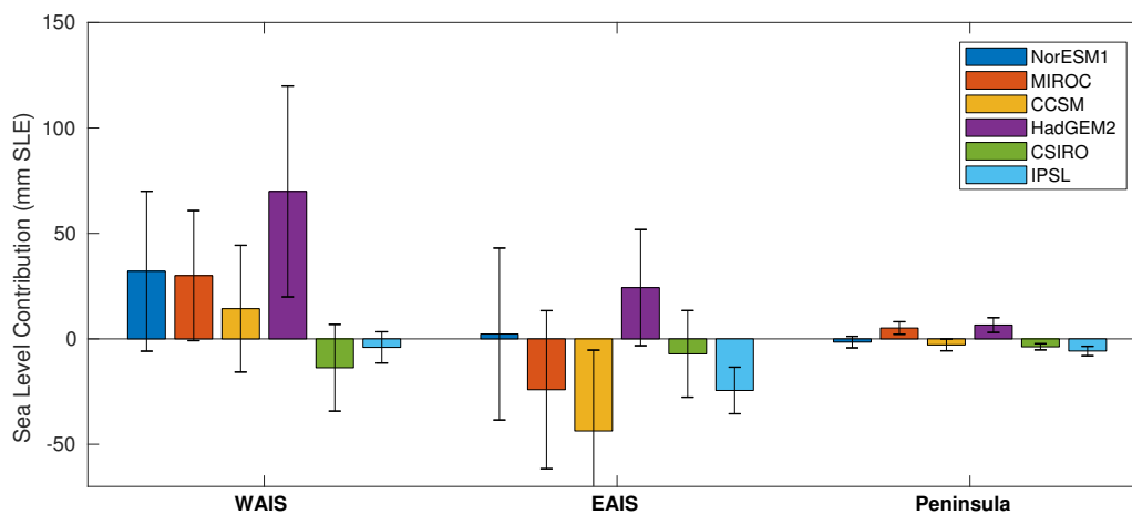
Figure 8. Regional change in volume above floatation (in mm SLE) for 2015–2100 from six CMIP5 AOGCMs under the RCP 8.5 scenario with median forcing, relative to ctrl_proj. Black lines show the standard deviation.
