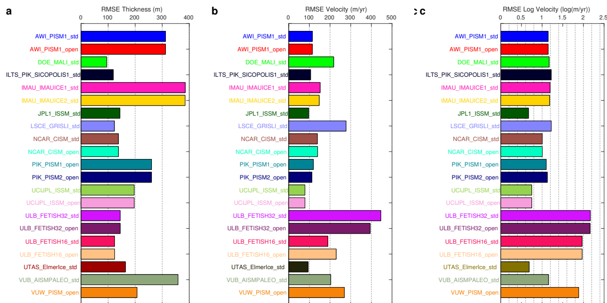
Figure 3. Root Mean Square Error in ice thickness (a, in m), ice velocity (b, in m/yr), and logarithm of ice velocity (c, in log(m/yr)) between modeled and observed values at the beginning of the experiments (January 2015).
