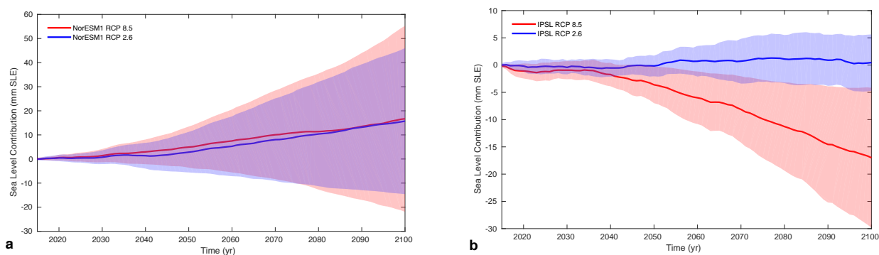
Figure 9. Impact of RCP scenario on projected evolution of ice volume above flotation for the NorESM1-M (a) and IPSL (b) AOGCMs. Red and blue curves show mean evolution for RCP 8.5 and RCP 2.6, respectively, and shaded background the standard deviation.
