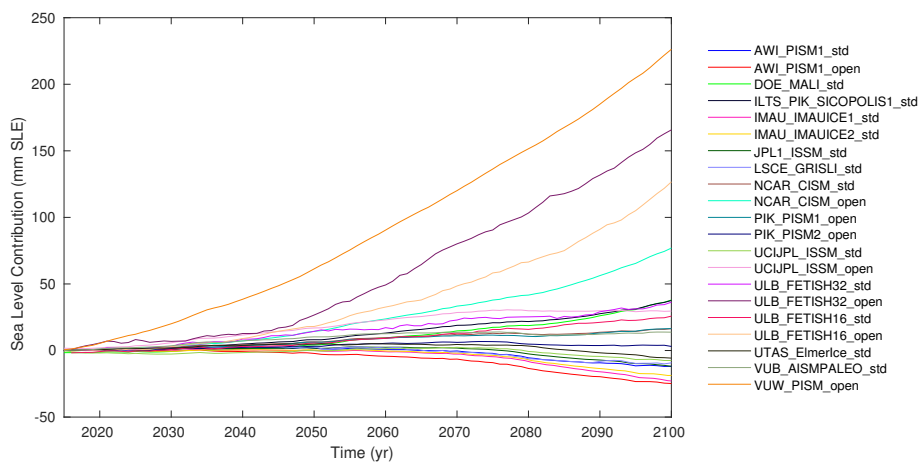
Figure 4. Evolution of ice volume above floatation (in mm SLE) over 2015–2100 from NorESM1-M RCP 8.5 scenario (exp01 and exp05) relative to ctrl_proj.
