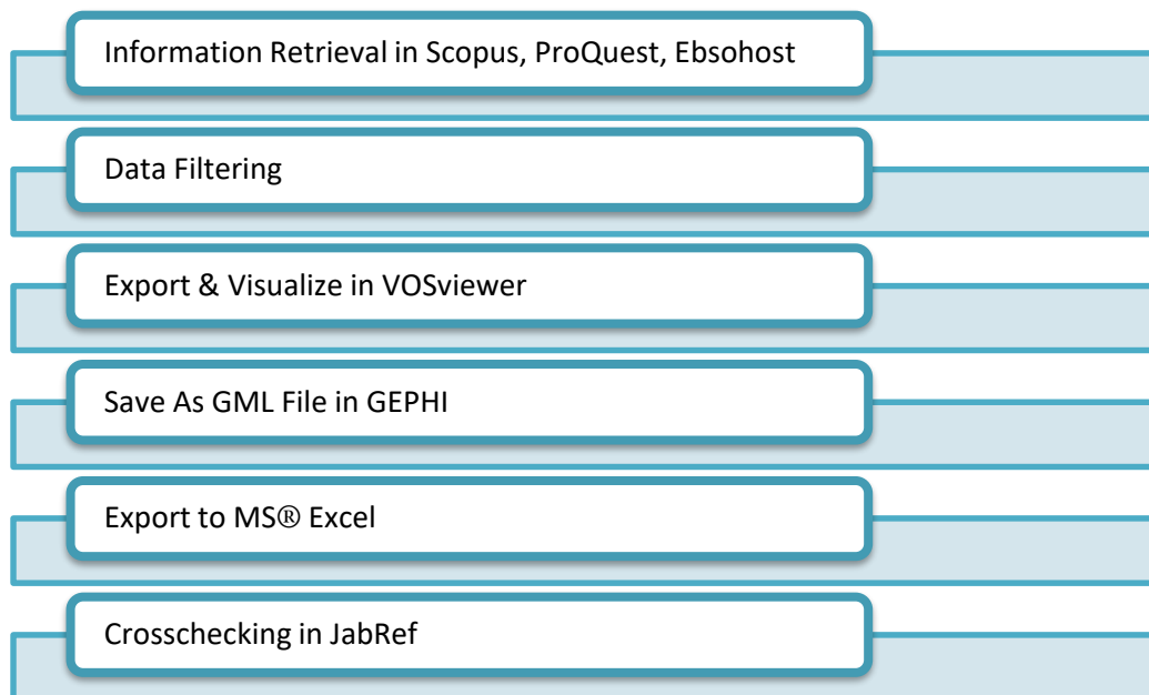
Figure 1: Research Flowchart
