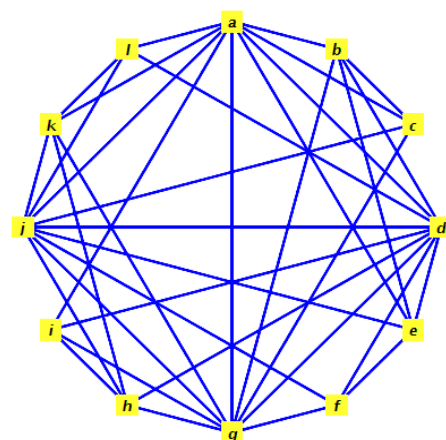
Figure 3: Compatibility Graph
