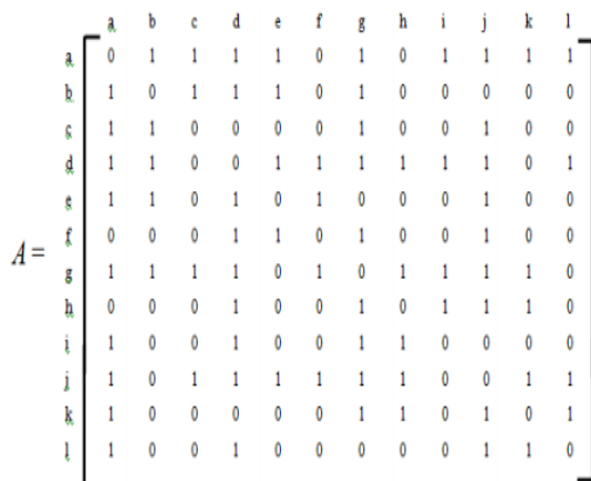
Figure 2: Matrix A
