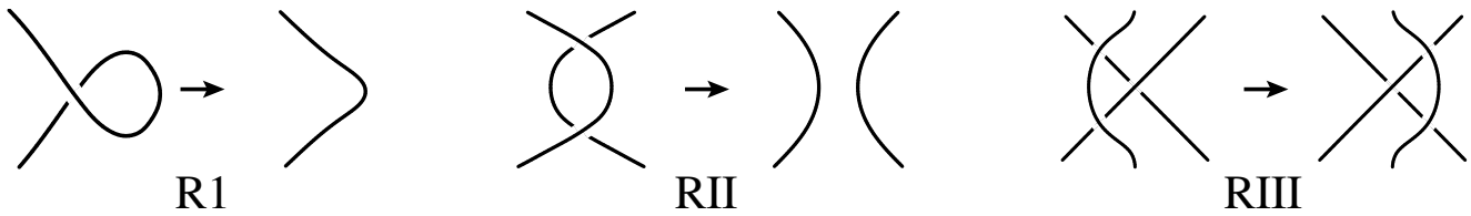
Figure 8 Reidemeister moves.
