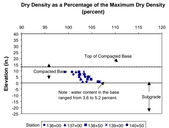
Figure 1 Dry Density Profiles for the Georgia Test Pads
