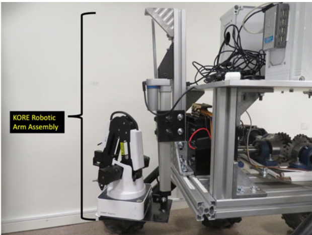
Fig. 16. Robotic arm assembly fixed to KORE chassis.
