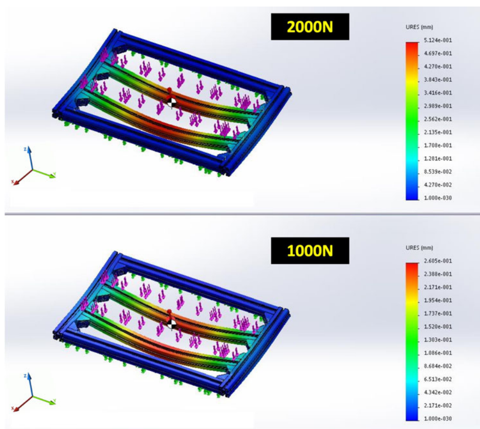
Fig. 7. Stress analysis of the aluminium frame along the XY-plane when subjected to distributed loads of 2000N (top) and 1000N (bottom). The colour scale shows the deformation in mm with red indicating maximum deformation zones and blue with the least deformation.
