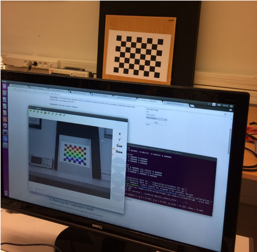
Fig. 14. The RGB-D camera was calibrated for both the RGB visual image and depth IR image using the checker-board of known dimensions. The calibration factor thus obtained is input into the algorithms to autocorrect offsets.
