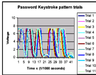
Fig 4. Training database of 11 trials for one password
