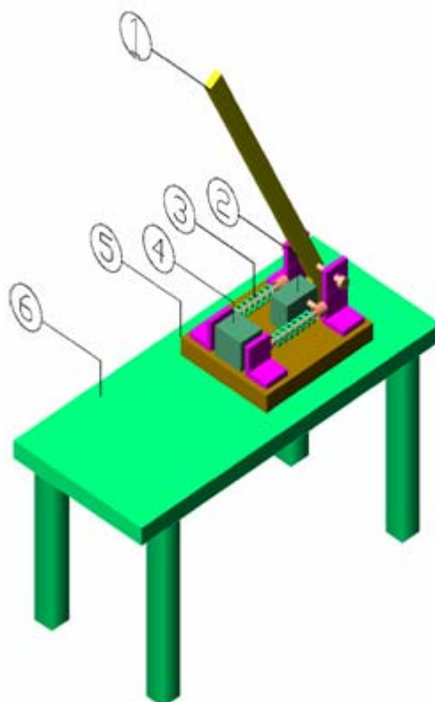
Figure 2. Isometric drawing of the Table mounted dika nut cracking device (1) control lever, (2) slider, (3) return spring (4) feed block (5) base plate (6) bench
