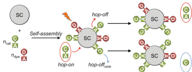
Fig. 9 Self-assembly of DSP system and hop-on/hop-off mechanism (shown for catalyst only); hop-on: unbound catalyst molecules occupy free surface sites through self-assembly; hop-off: desorption of catalyst from the particle surface; hop-off core : loss of catalyst core from the particle surface (anchoring group stays on surface). SC = semiconductor; C = catalyst; D = dye; A = anchoring group. 30
