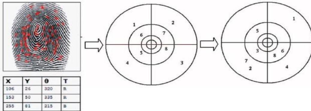
Figure 8: Polar transformation where every sector is mapped to other randomly selected sector (Ratha et al.)
