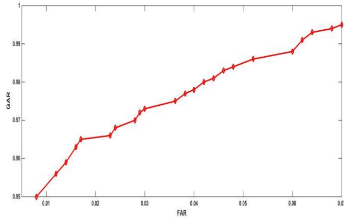
Fig. 14. ROC curve
