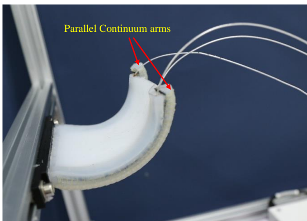
Fig. 14. The final curved shape of the manufactured soft surface in the test rig under static conditions it has been actuated by a pair of parallel continuum arms (Test 2) bending into a curvature of radius r=0.092 m.
