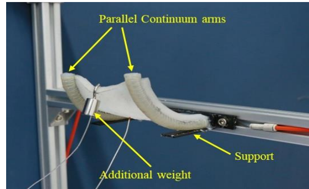
Fig. 17. Image of the experimental test of the actuated flexible surface undergoing an additional weight positioned between two embedded continuum arms.
