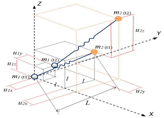
Fig. 3. Representation of two typical interconnected lumped masses of the model before deformation (at t=t_1 ) and after that (at t=t_2 )
