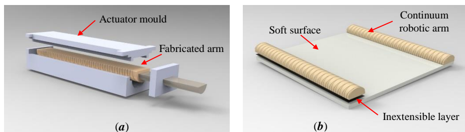
Fig. 10. a) The actuator mould designed to fabricate continuum arm; b) Schematic details of the integrated surface-actuator used in the experimental test rig.
