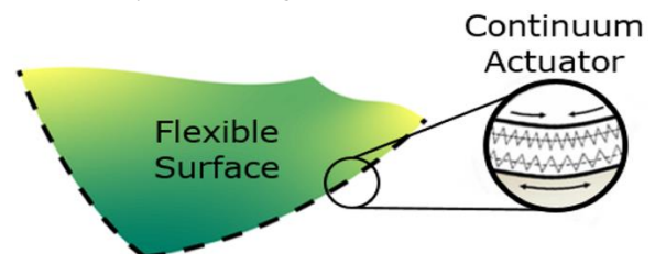
Fig. 1. A representative LDCS deformed into multiple curvatures using actuating elements placed on the surface edge
