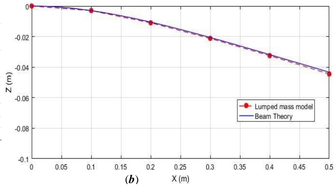
Fig. 4. a) Representation of a 3D, beam model under its weight composed of 24 lumped masses interconnected by linear springs. b) Results of the model deflection versus the beam theory
