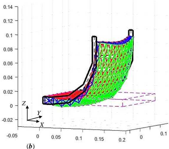
Fig. 8. Test 2- The LDCS model deformed by a pair of continuum arm attached to two parallel sides when bending into a curvature of radius r=0.092 m ( k_t=10.87 m -1 ); a) top-layer view b) bottom-layer view.
