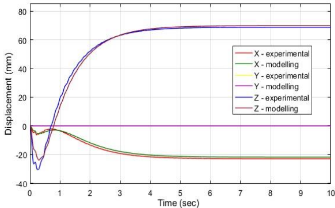
Fig. 19. Comparing the dynamic behaviour of the modelled LDCS and the empirical surface through recording the displacement of point P_4 as indicated in Fig. 12 over time in the 3 directions X , Y , and Z .
