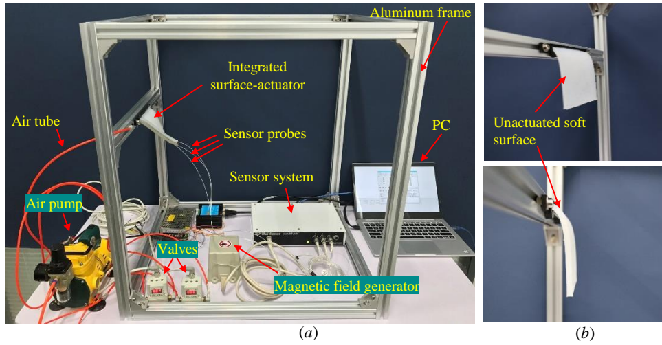
Fig. 9. a) The test rig set up for the experimental tests; b) two different views of the manufactured soft surface without integrated actuator and sensors while clamped at one edge hanging under gravity.
