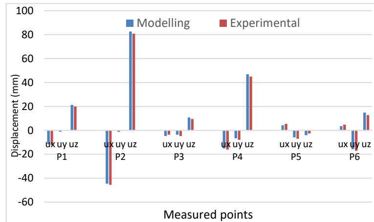
Fig. 15. Comparison of displacement results between the LDCS model and the experimental surface at 6 measured points in Test 1. [Data acquired from Table1.]
