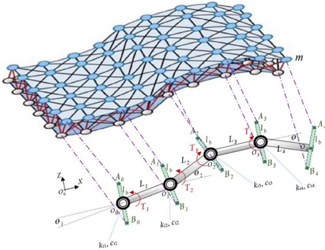
Fig. 6. Representation of the LDCS integrated with an arm model along one side of the surface.
