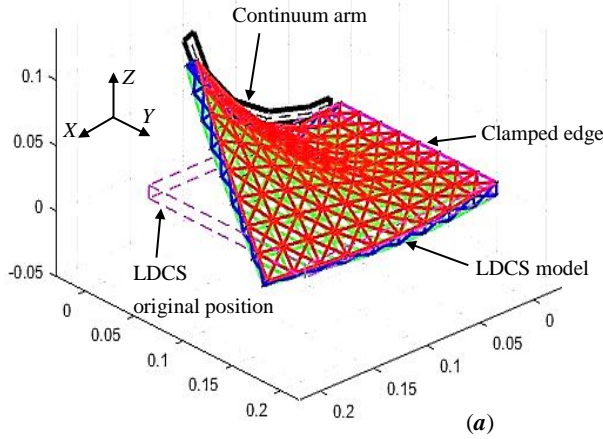
Fig. 7. Test 1- The LDCS model deformed by a single continuum arm when it bends into a curvature of radius r=0.131 m ( k_t=7.63 m -1 ), shown in two different views (a and b).
