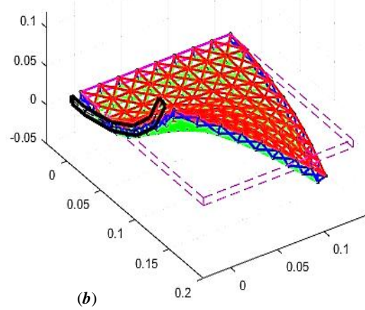
Fig. 7. Test 1- The LDCS model deformed by a single continuum arm when it bends into a curvature of radius r=0.131 m ( k_t=7.63 m -1 ), shown in two different views (a and b).
