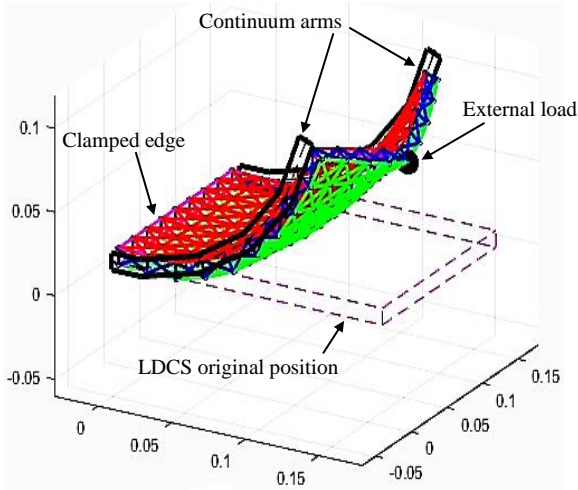
Fig. 18. Simulation results for the lumped mass LDCS model undergoing a concentrated external force displayed at its final static deformed shape after actuation by two continuum arms embedded in its two parallel edges.
