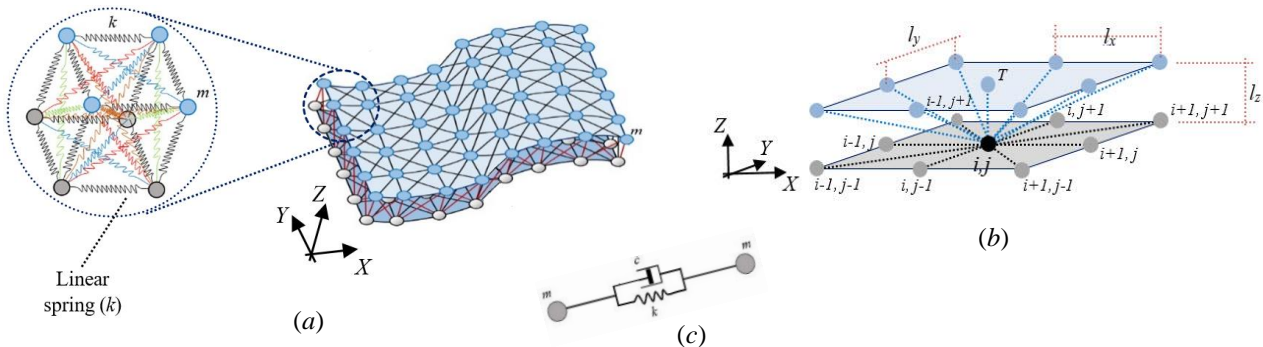
Fig. 2. a) Representation of the LDCS lumped-mass model with a close-up view of one corner; b) Arrangement of the masses linking to the typical central mass i,j in bottom layer of the 2-layer model; c) The featured spring-damper link connecting every two masses in the model
