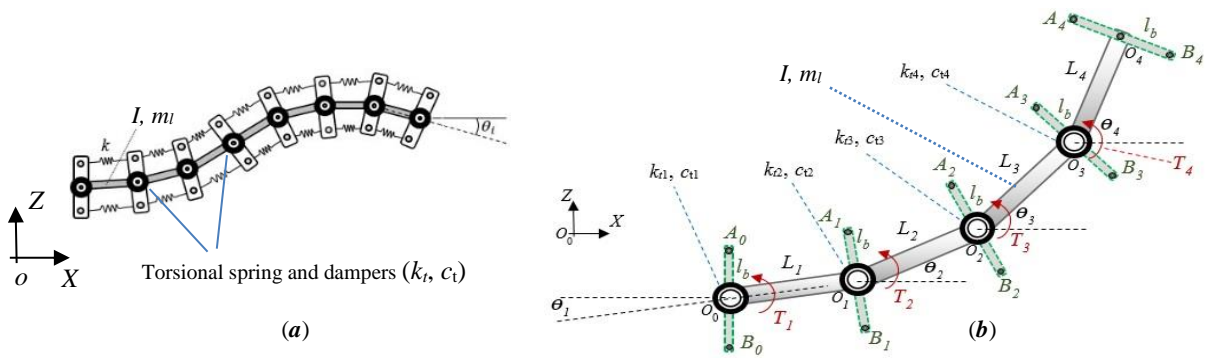
Fig. 5. a) Schematic of general arm model when embedded in the flexible LDCS; b) The lumped parameter, multibody actuator model to match the 2-layer configuration of the flexible LDCS in which k_i and c_i denote stiffness and damping coefficients of torsional springs and torsional dampers respectively. The torques T_r (where r=1, 2, 3, 4 ) are applied on the left-hand joints of the links at O_0, O_1, O_2 , and O_3 causing the rotations ( \theta_i ) of the four main links L_1, L_2, L_3 , and L_4 to generate a desired curvature throughout the arm. Likewise, transverse links A_1B_1, A_2B_2, A_3B_3 , and A_4B_4 , all with the equal length of |A_iB_i| = l_b , are attached and perpendicular to the main links.
