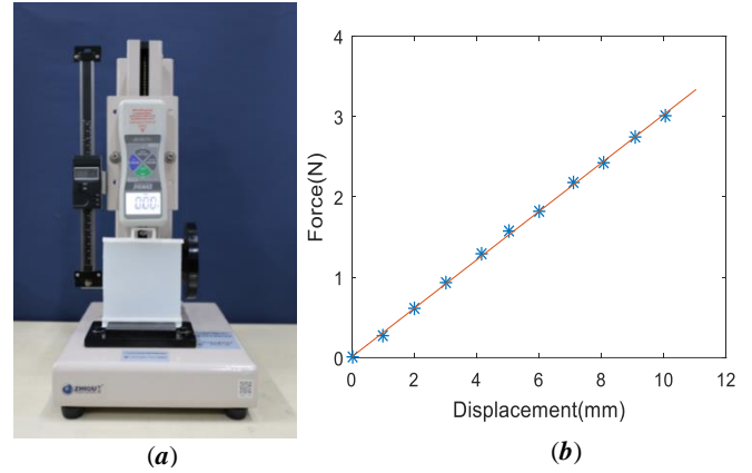
Fig. 11. a) A tensile test machine applying uniform axial force to the soft surface; b) The resulted force-displacement graph to calculate Young's modulus of the surface.
