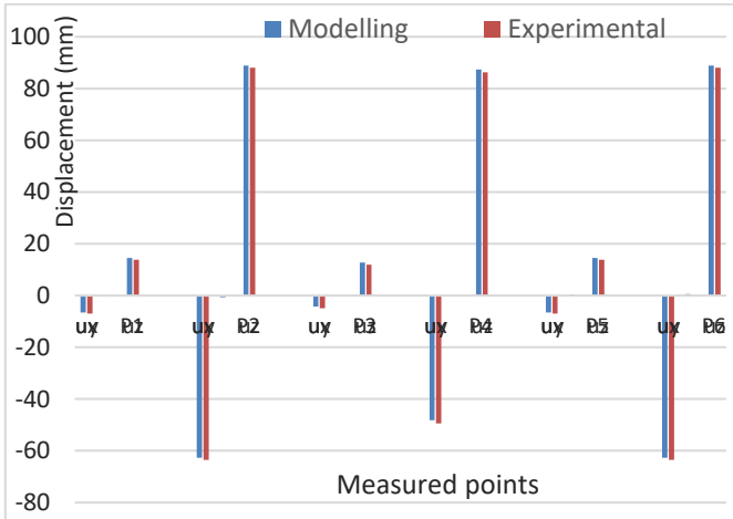
Fig. 16. Comparison of displacement results between the LDCS model and the experimental surface at 6 measured points in Test 2. [Data acquired from Table 2.]
