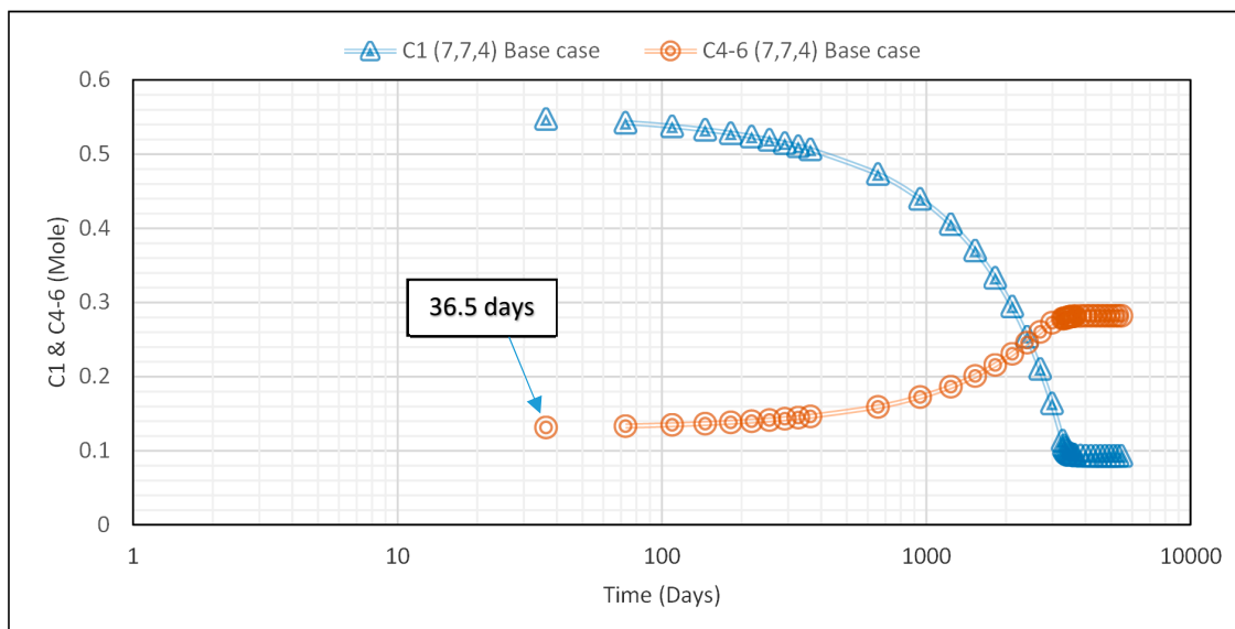
Figure 6. Composition of fluid components over time for the base case at the wellbore.
