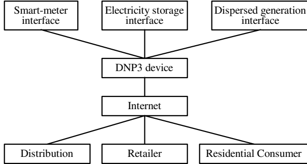
Fig. 3. Cyber-security example of a single DNP3 outstation device with multiple masters.
