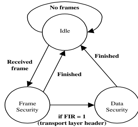
Fig. 1. Cyber-security states.
