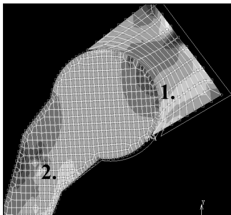
Figure 7 - Current FEA results showing contact forces, displacement and neck stress.
