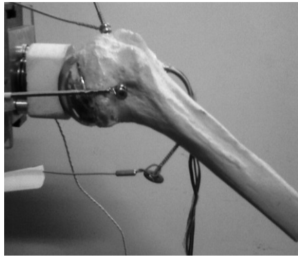
Figure 4 – Copeland Implanted with strain gauges.
