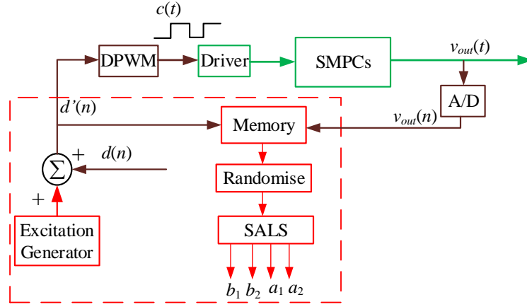
Fig.11. Open Loop SALS Estimation Scheme.
