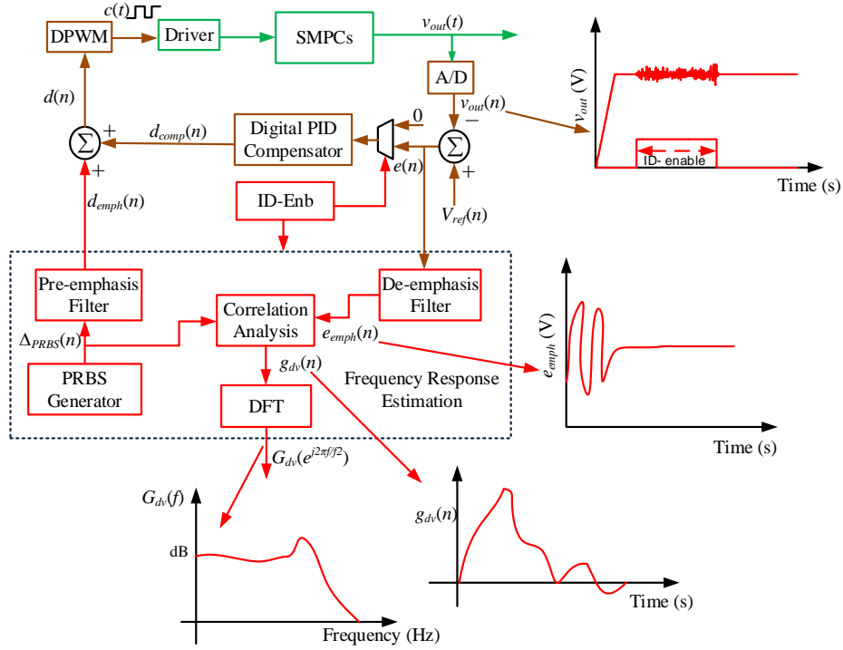
Fig. 13. Non-parametric correlation block diagram.
