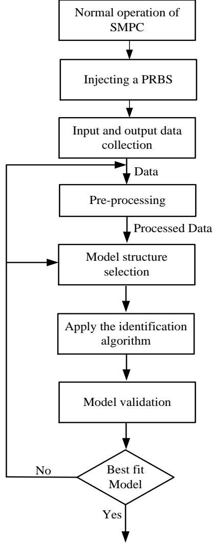
Fig. 5. Parametric identification procedure of SMPC.
