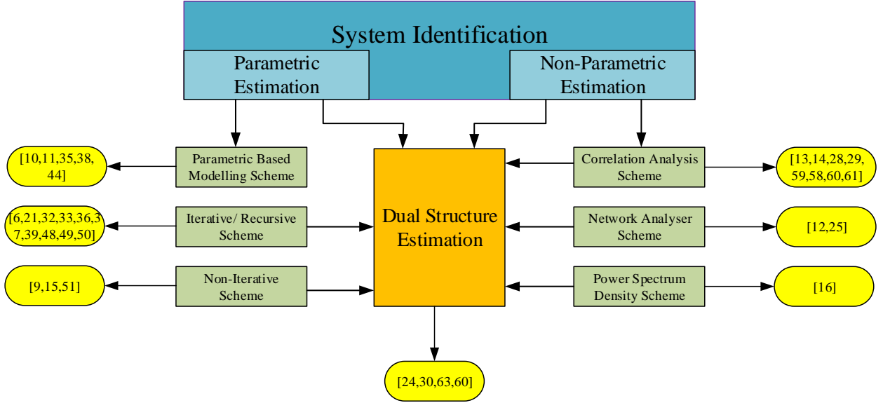
Fig.1. Advances in system identification for SMPCs.
