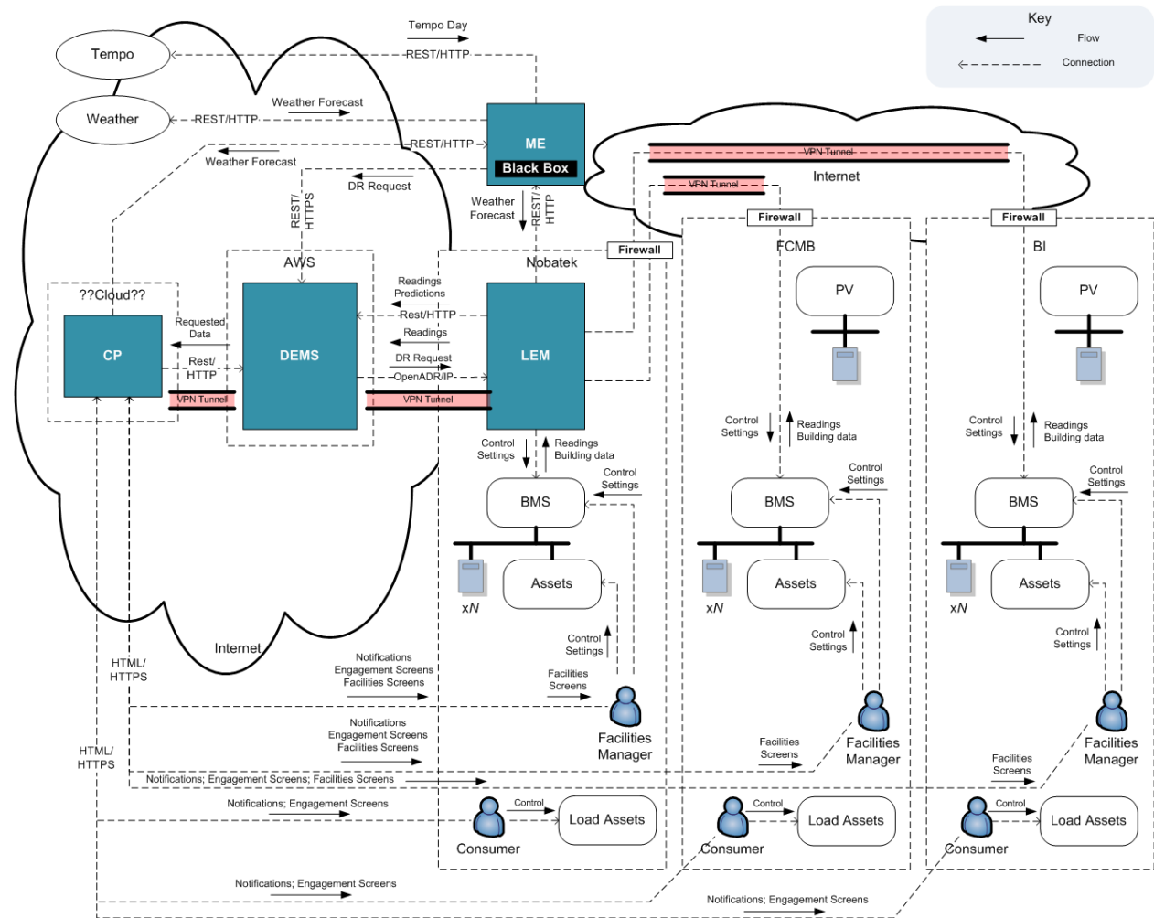
FIGURE 4: ANGLT PILOT SITE CONFIGURATION
