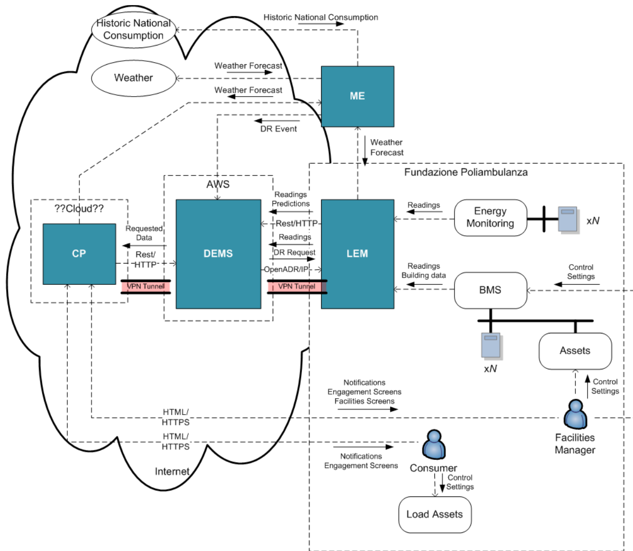
FIGURE 5: BRESCIA PILOT SITE CONFIGURATION
