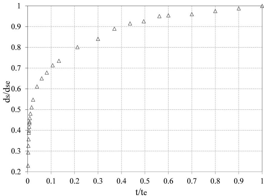
Figure 3. Time required for the expansion of the scour for a pier without a collar.
