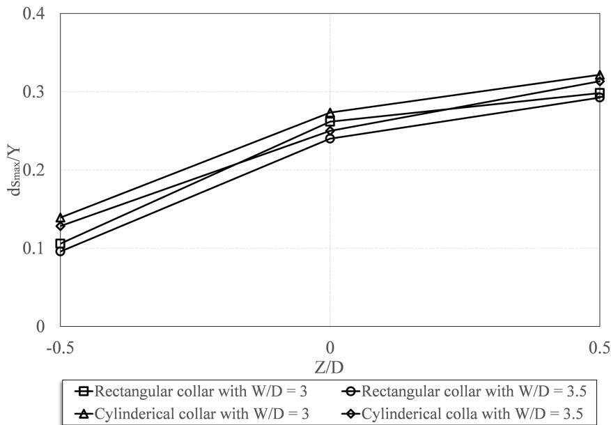
Figure 6. Comparison of the performances of the circular and the rectangular collars. doi:10.1371/journal.pone.0098592.g006
