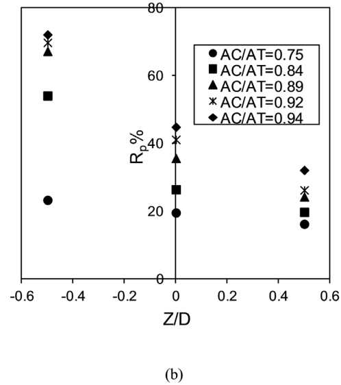
Figure 8. The effect of non-dimensional parameters of a circular collar on percentage reduction; a) A_c/A_T b) Z/D . doi:10.1371/journal.pone.0098592.g008
