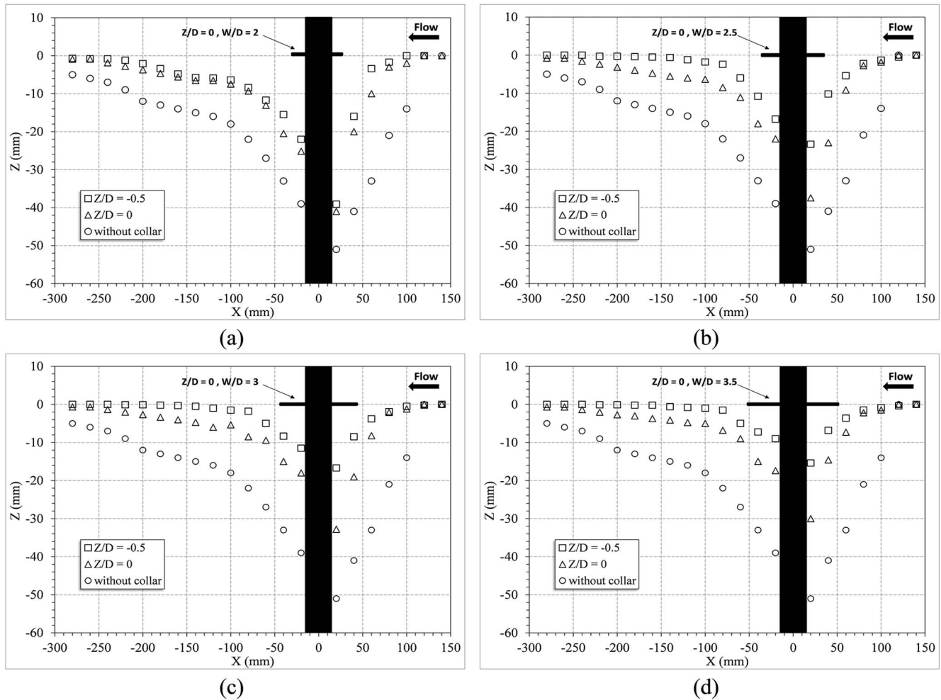
Figure 4. Longitudinal profiles of the bed changes around the bridge pier with the circular collars: a) W/D=2 , b) W/D=2.5 , c) W/D=3 , d) W/D=3.5 (scale, 1:5).
