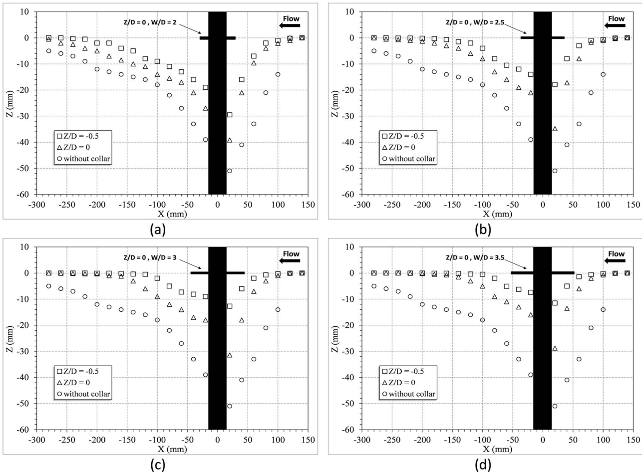
Figure 5. Longitudinal profiles of the bed changes around the bridge pier with the rectangular collars: a) W/D = 2 , b) W/D = 2.5 , c) W/D = 3 , d) W/D = 3.5 (scale, 1:5). doi:10.1371/journal.pone.0098592.g005
