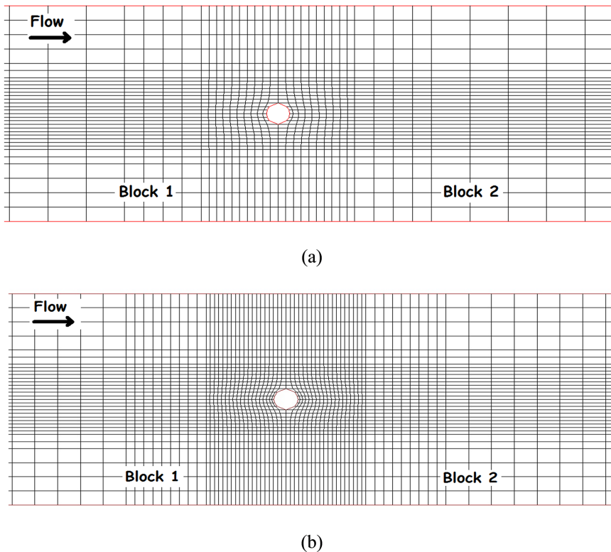
Figure 7. Two developed grids in SSIIM 2.0 grid editor for a single bridge pier. doi:10.1371/journal.pone.0098592.g007
