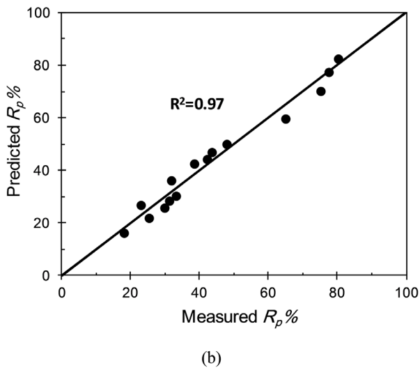
Figure 9. Comparison of measured and predicted values for a) a circular collar and b) a rectangular collar. doi:10.1371/journal.pone.0098592.g009
