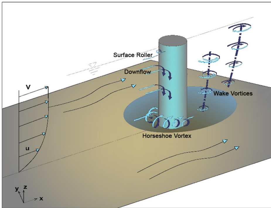
Figure 1. Flow and scour pattern around a cylindrical pier.
