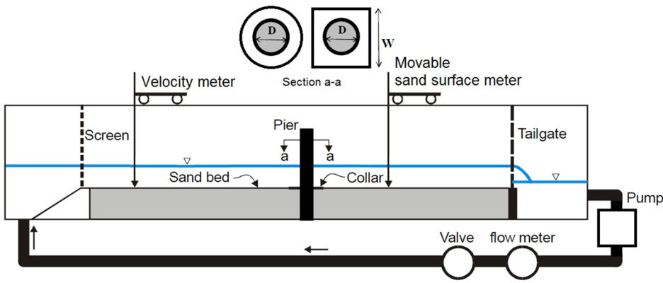
Figure 2. Schematic view of the experimental flume and single bridge pier.
