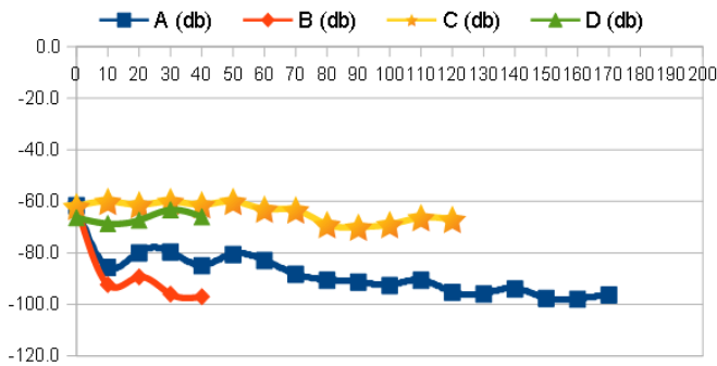
Figure 4: Bluetooth and ZigBee attenuation at zero obstacles
