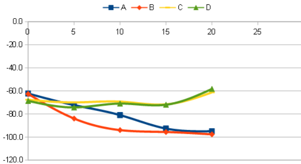
Figure. 6: Bluetooth and ZigBee attenuation at thick foliage
