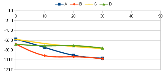
Figure 5: Bluetooth and ZigBee attenuation with mild obstacles
