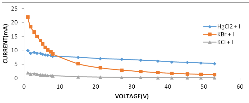
Figure 5g. I-V curve for C.acuminata , L.arboreus & B.spectabilis dye in Sunny weather Degeneration in DSSC
