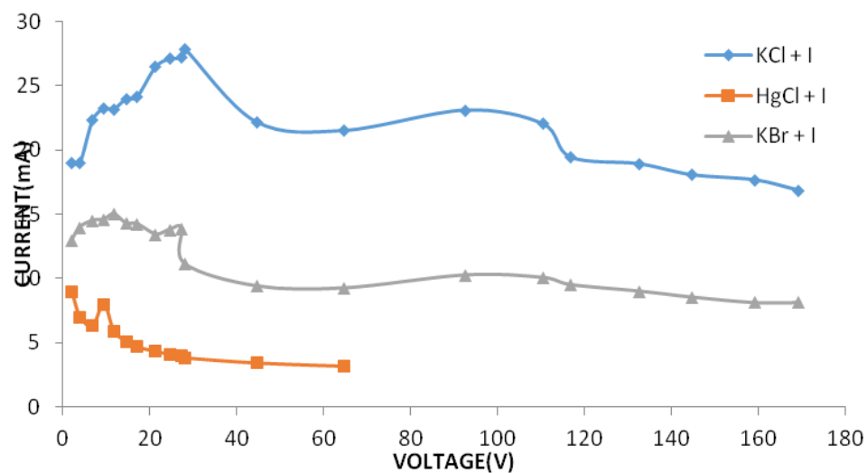
Figure 5(a). I-V curve for C.acuminata & B.spectabilis dye Indoor
