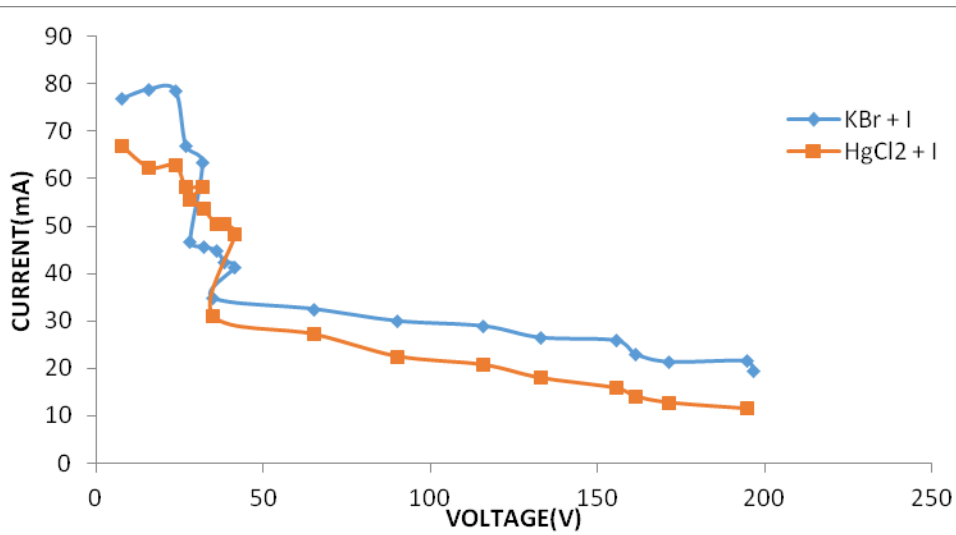
Figure 2(b). I-V curve for C.acuminata dye Indoor
