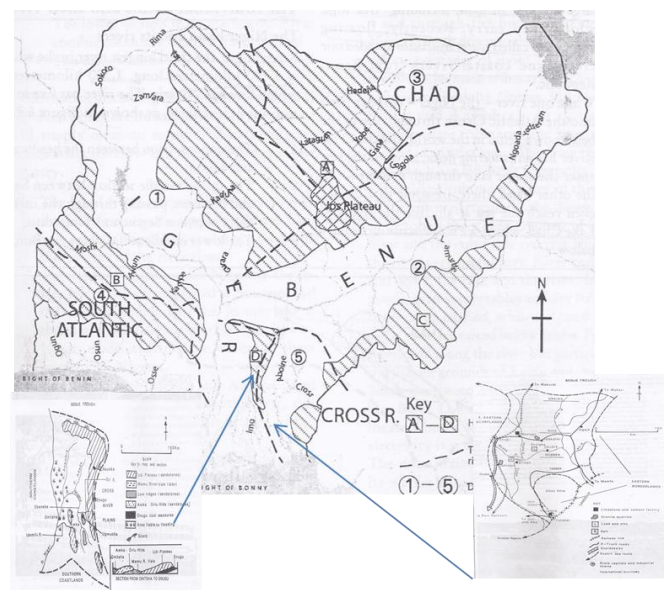
Figure 1: Map of Nigeria showing Udi Escarpment and the
