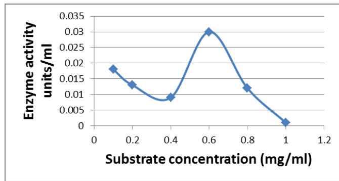
Fig. 15. Effect of substrate concentration (0.6% carboxymethyl cellulase) on the activity of partially purified cellulase obtained from the Roma vf variety of tomato fruits infected by A. niger .
