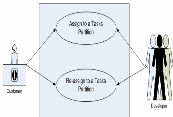
Fig. 1 Tasks Assignment
