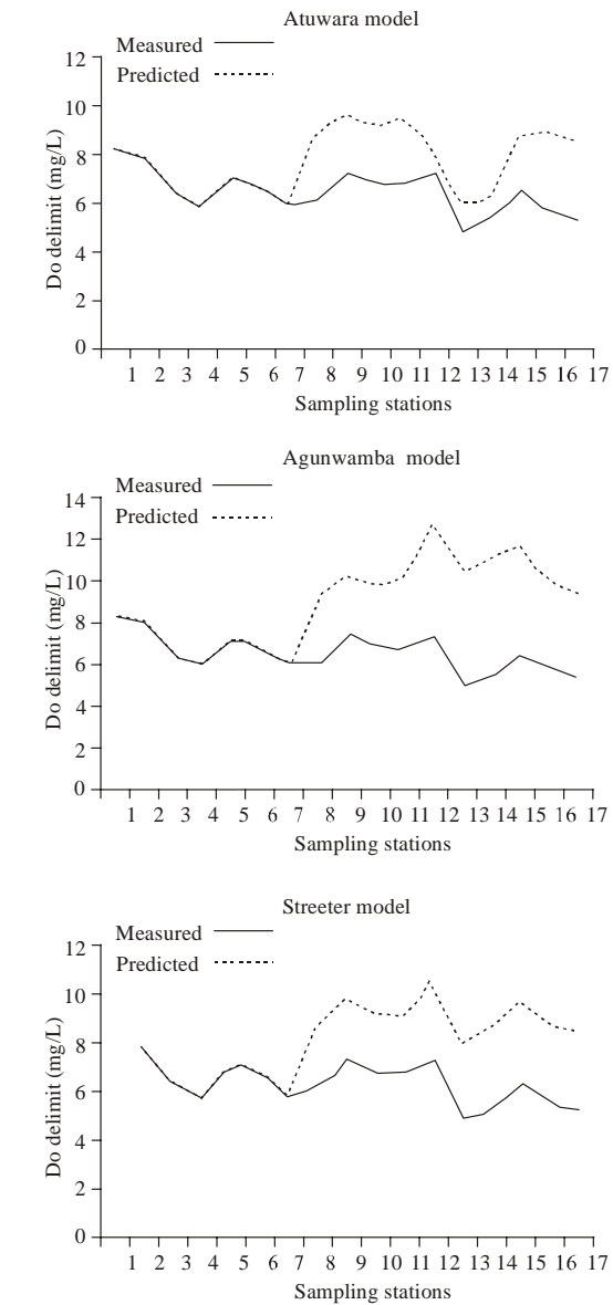
Fig. 4: DO deficit plot against sampling stations using the modified Streeter-Phelps equation (July data)
