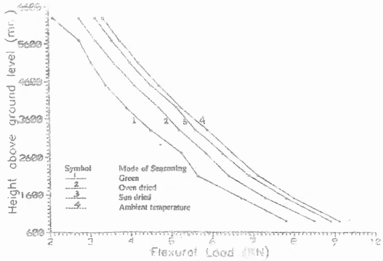
Fig. 4: Variation of Ultimate Flexural Load along the Length of Bamboo Culm
