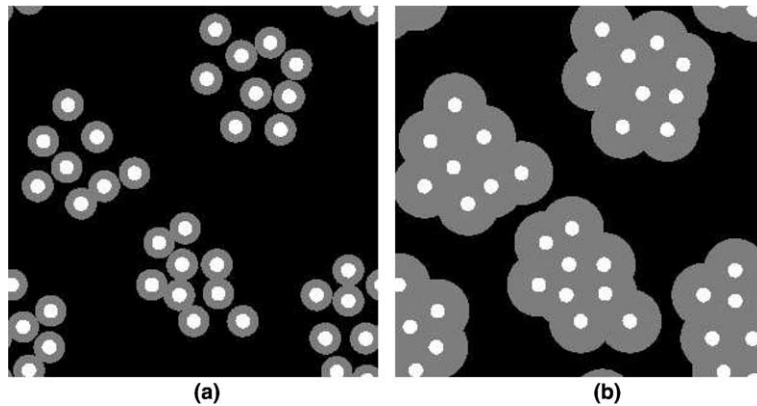
Fig. 18. Result of the threshold operation performed on the distance function: (a) d_0 = 0.023 and (b) d_0 = 0.066 .
