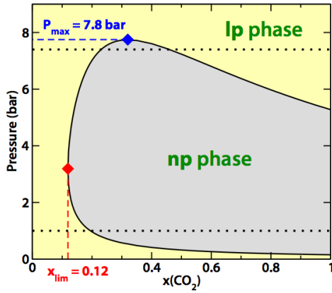
Figure 1: Predicted diagram of stability of the np and lp phases of MIL-53 (Al) upon adsorption of a CO 2 /CH 4 mixture at 304 K, as a function of total pressure and mixture composition. The horizontal dotted lines correspond to the constant-pressure experiments. 7
