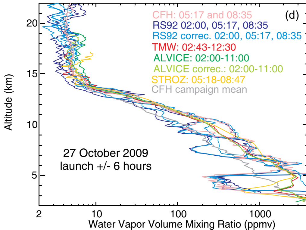
Fig. 5c and d. Balloon-borne and lidar water vapor profiles measured on various campaign nights (with various coincidence criteria applying). Lidar integrated for several hours with a \pm 6 h coincidence criterion with balloon measurements. See text for details.
