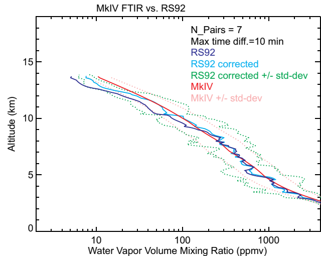
Fig. 10. Campaign-mean water vapor mixing ratio profiles, and standard deviations, measured simultaneously by the ground-based FTIR MkiV and the Vaisala RS92 PTU radiosondes (7 coincidences).
