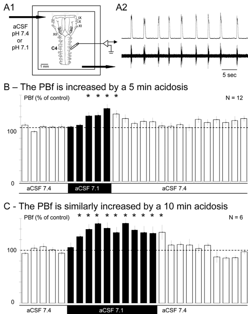
Figure 1. Acidosis increases the phrenic burst frequency of en bloc medullary preparations. A – Schematic presentation of the en bloc preparation of neonatal mice (A1) and example of raw and integrated phrenic bursts (bottom and top traces, respectively) produced by the isolated respiratory rhythm generator (RRG) on the C4 ventral roots of en bloc preparations (A2). B – Columns of the histogram show the mean (and SEM) phrenic burst frequency (PBf; expressed as % of the control PBf) measured every min (one column = 1 min) in 12 en bloc preparations when the control aCSF(7.4) (white columns) superfusing the preparations was replaced by aCSF(7.1) for 5 min (black columns). Note that acidosis significantly increased the PBf (asterisks indicate a p < 0.05 statistical difference). C- As in B but aCSF(7.1) application for 10 min to 6 other preparations. Note that the PBf reached a plateau from the 5 th to the 10 th min of aCSF(7.1) application. doi:10.1371/journal.pone.0013644.g001
