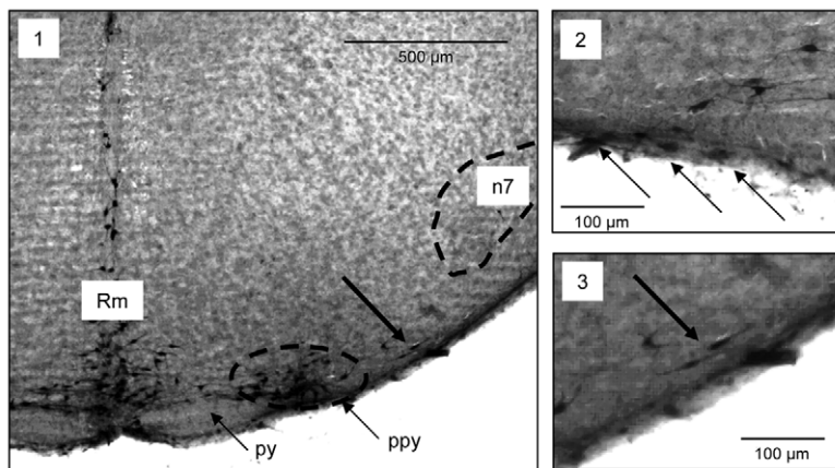
Figure 3. SERT mRNA and 5-HT-containing neurons in the vicinity of the RTN/pFRG of neonatal mice. A: Two serial coronal sections passing through the RTN/pFRG area of a neonatal mouse show SERT mRNA expression (A1) and Cresyl Violet staining (A2). Anatomical limits drawn from A2 Cresyl Violet section have been superimposed on A1 section (dotted line). Note SERT mRNA is expressed in three areas, the median Raphe Magnus (Rm), the para-pyramidal group (ppy) lateral to the pyramidal tract (py) and a lateral spot (arrow) located in a medio-ventral position from the facial motor nucleus (n7), as defined from Cresyl Violet staining (in A2). B- 5-HT neurons in the RTN/pFRG area of a neonatal mouse. Note 5-HT neurons in the median raphe magnus (Rm), the parapyramidal group (ppy, dotted circle) lateral to the pyramidal tract (py) and the lateral spot (arrow in B1) in the medio-ventral location of the facial nucleus (n7). In B2 and B3, note the superficial location of some 5-HT neurons (arrows). B3 is an enlargement of B1.
