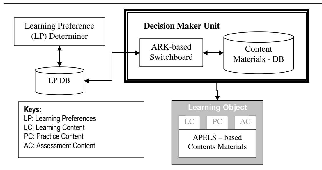
Figure 33: A high-level design view of an Adaptable Personalised E-Learning System (A L PELS)
