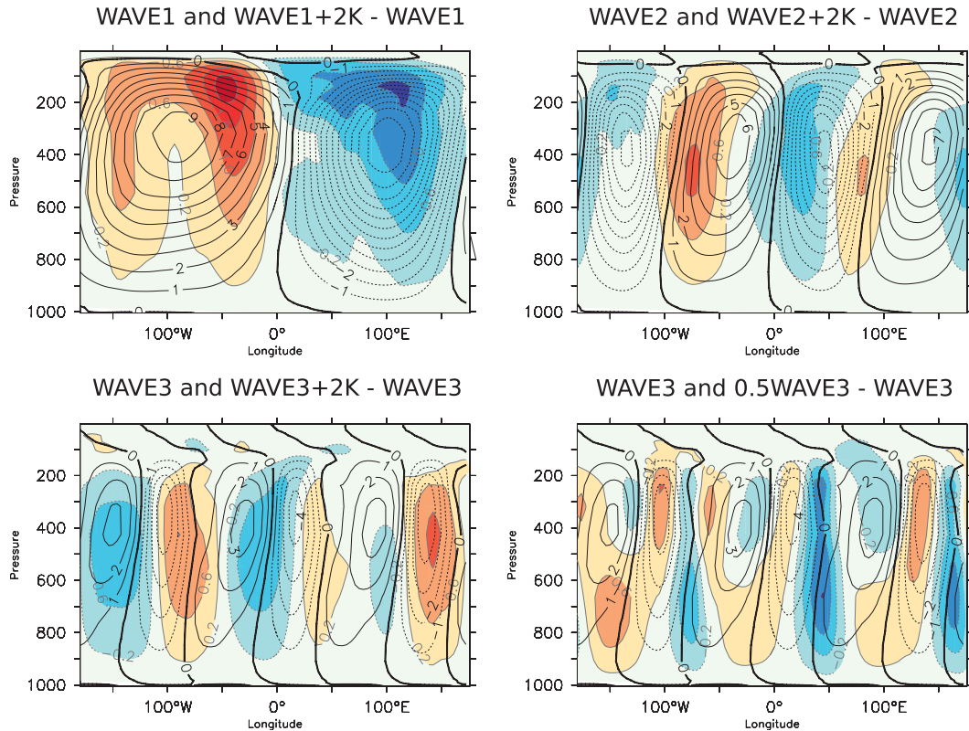
FIG. 7. As in Fig. 6, but for mean zonal streamfunction anomalies over the domain of the Hadley cells.
