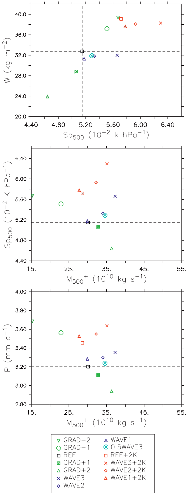
FIG. 9. Scatterplots illustrating the mean thermodynamic state of the tropical atmosphere: (top) column-integrated water vapor W vs 500-hPa dry static stability S_{p500} , (middle) dry static stability at 500 hPa vs mean ascending midtropospheric velocity M_{500}^+ , and (bottom) precipitation P vs mean ascending midtropospheric velocity M_{500}^+ . All variables are averaged over the domain of the Hadley cells.
