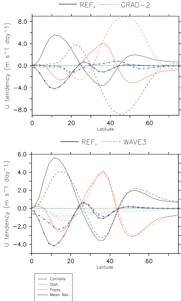
FIG. 10. Zonal-mean zonal wind balance at the 200-hPa height and the contribution to wind tendency ( \text{m s}^{-1} \text{ day}^{-1} ) from the mean advection, Coriolis torque, and stationary and transient eddies. The continuous lines designate the results for the simulation REF; dashed lines indicate the results of the simulations (top) GRAD-2 and (bottom) WAVE3.
