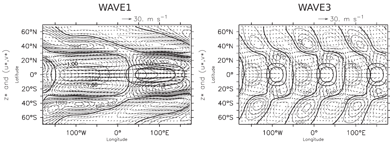
FIG. 5. Geopotential anomalies (m, contours), the anomalous flow at the 200-hPa level ( \text{m s}^{-1} , vectors), and longitudinal SST anomalies (K, thick contours) for the simulations (left) WAVE1 and (right) WAVE3.
