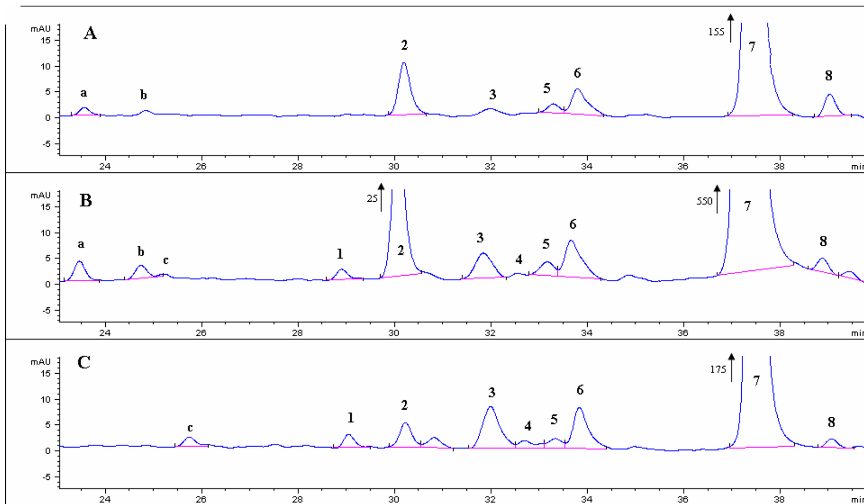
566 567 Figure 2: HPLC chromatograms at 450nm of the carotenoids of Resisto slices before drying (A), after drying (B) and after 120 days 568 storage (C). a: Possibly \beta -carotene-5,6,5',6'-diepoxide (23 min.) (414; 440 ; 468nm); b: Possibly \beta -carotene-5,6,5',8'-diepoxide (24 min.) (400; 422 ; 450nm); c: 569 unidentified (25 min.) (406; 424 ; 450nm); 1: Possibly 13-cis- \beta -carotene-5,6 epoxide (29min.) (main wavelengths: 416; 439 ; 476nm); 2: Possibly \beta -carotene-5,6 epoxide 570 (30min.) (422; 446 ; 472nm); 3: Possibly \beta -carotene-5,8 epoxide (32min.) (406; 428 ; 452nm); 4&5: Unidentified; 6:13-cis \beta -carotene (34min.) (338;422; 444 ; 472nm); 7: All- 571 trans- \beta -carotene (37min.) ( 452 ; 478nm); 8: Possibly 9 cis- \beta -carotene (39min.) ( 446 ; 472nm). The three graphs are not to the same scale because of differing dry matter 572 contents (respectively 27%, 89% and 87%). The graphs have been scaled to illustrate the minor peaks and therefore the larger peaks have been truncated.
