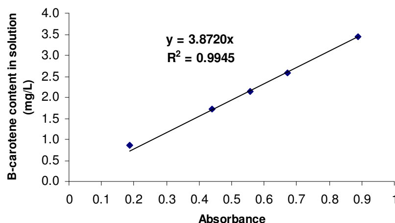
Figure 2-2: β-carotene standard curve at 450nm absorbance using a UVIKON 933 Spectrophotometer, France
