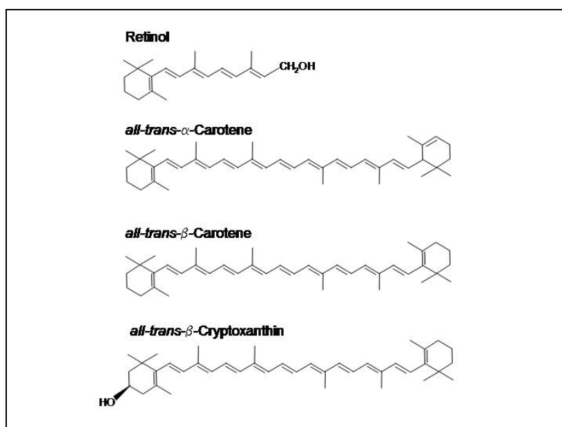
Figure 1-11: Structures of the most common provitamin A carotenoids and retinol. National Academy of Sciences/Institute of Medicine (2001).
