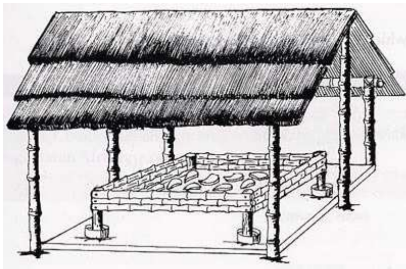
Figure 1-7: Shade dryer. FAO (2001).
