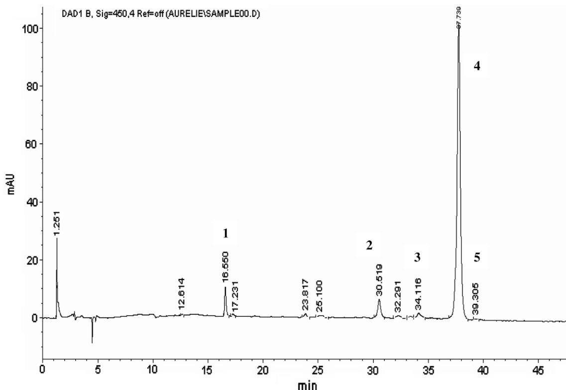
Fig. 5. Reverse phase HPLC separation of carotenoids in raw sweetpotatoes. 1, non-identified polar carotenoid; 2, \beta -carotene 5,6 epoxide; 3, 13- cis - \beta -carotene; 4, all trans - \beta -carotene and 5, probably 9- cis - \beta -carotene.
