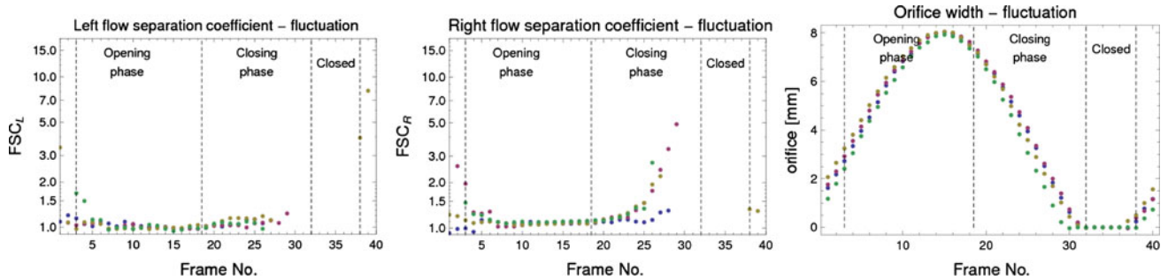
Fig. 12 Fluctuation of the left and right flow separation coefficients and of the orifice width. Measurements 012s-w ( Re = 5,400 , with glottal closure). Dashed lines delimit the boundaries of vocal fold vibration phases ( opening phase , closing and closed phase )
