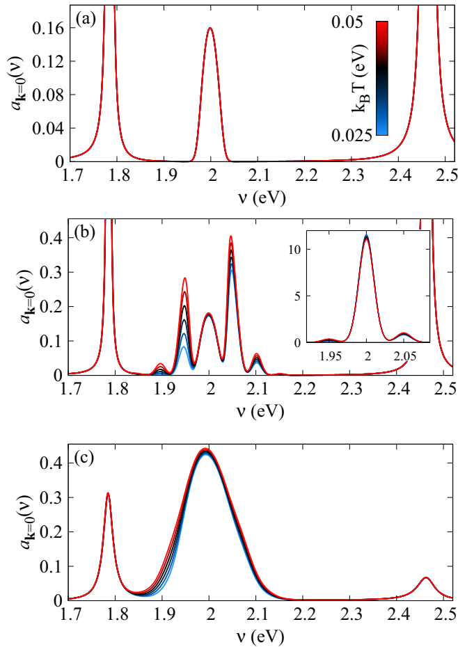
FIG. 4. Evolution of absorption spectra with the temperature (values shown on the color scale) for the following: (a) A system with no coupling to vibrational modes, S = 0 ; in this case all lines lie on top of one another since there is no temperature dependence. (b) Coupling to a single vibrational mode with S = 0.06 , \Omega = 0.05 eV. The inset shows the bare molecular spectrum. The height of the absorption spectra increases with increasing T in the main panel; the opposite occurs in the inset. (c) Including the effects of cavity losses and nonradiative excitonic decay. Again the absorption spectra increases with increasing T . All panels are for g\sqrt{N} = 0.3 eV, and other parameters as in previous figures.
