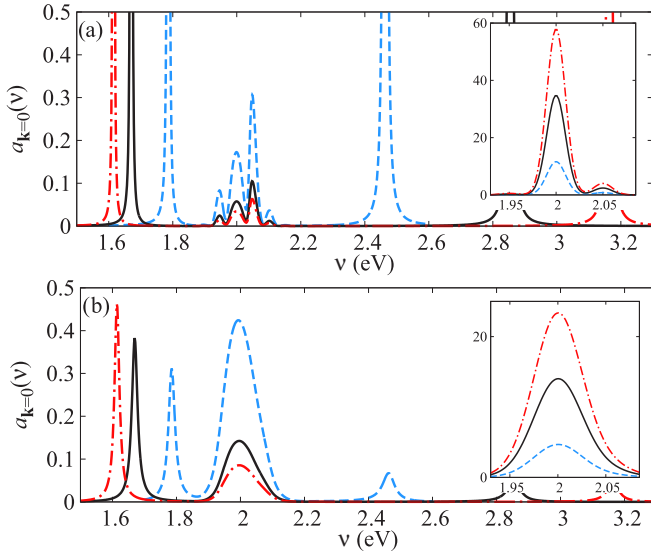
FIG. 3. The evolution of absorption spectra with the strength of g\sqrt{N} for a system with a single vibrational mode with S = 0.06 , \Omega = 0.05 eV. The insets show the equivalent absorption spectra for bare molecules. The other parameters are as in Fig. 1. Panel (a) shows the spectrum for a perfect cavity while panel (b) includes the effects of cavity losses and nonradiative excitonic decay exactly as in Fig. 1(b).
