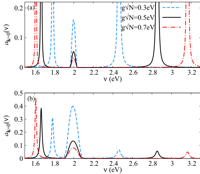
FIG. 1. Evolution of \mathbf{k} = 0 absorption spectrum, a(v) for various values of the polariton splitting g_{\mathbf{k}=0} = \sqrt{N_m} for the system with no auxiliary degrees of freedom. Plotted for k_B T = 0.025 eV (i.e., T = 290 K), f = 0.05 , \omega_{\mathbf{k}=0} = 2.1 eV, and a truncated Gaussian distribution of excitonic energies h(\epsilon) \propto \Theta(\epsilon) e^{-(\epsilon - \epsilon_0)^2 / 2\sigma^2} with \epsilon_0 = 2.0 eV, \sigma = 0.01 eV. Panel (a) shows the results with a perfect cavity while (b) includes the effects of cavity losses at rate \kappa = 0.075 eV and excitonic nonradiative decay at rate \gamma = 10^{-4} eV; also the width of the energy distribution is larger, \sigma = 0.025 eV as discussed in Appendix A.
