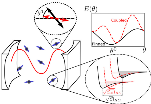
FIG. 2. Schematic diagram showing orientational and vibrational degrees of freedom. The top right inset shows the potential-energy landscape with (dashed red line) and without (solid black line) a cavity. The other insets show (top) the orientational degree of freedom and (bottom right) the vibrational degree of freedom illustrating how the coupling to light decreases the displacement between the ground and excited manifolds. Shifts due to coupling to the cavity are exaggerated for clarity in all three insets.
