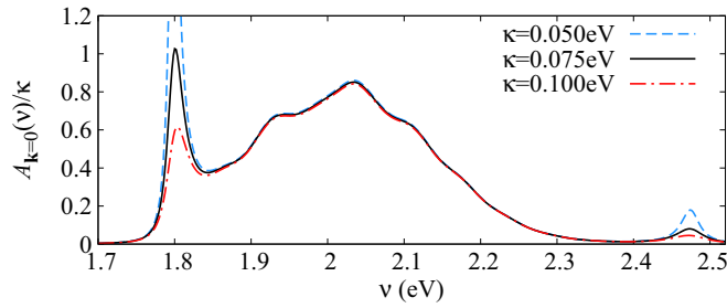
FIG. 6. Absorption spectrum, as defined by the full expression, Eq. (A4), plotted for S_1 = 0.25 , S_2 = 0.35 , \Omega_1 = 0.06 eV, \Omega_2 = 0.05 eV, k_B T = 0.035 eV, and various cavity loss rates \kappa . Other parameters are as in Fig. 5. As discussed in the text, in order that the polaritonic peaks have a finite width, one must include the effects of excitonic absorption or nonmirror cavity losses. For this figure, we include an excitonic linewidth \gamma = 10^{-4} eV.
