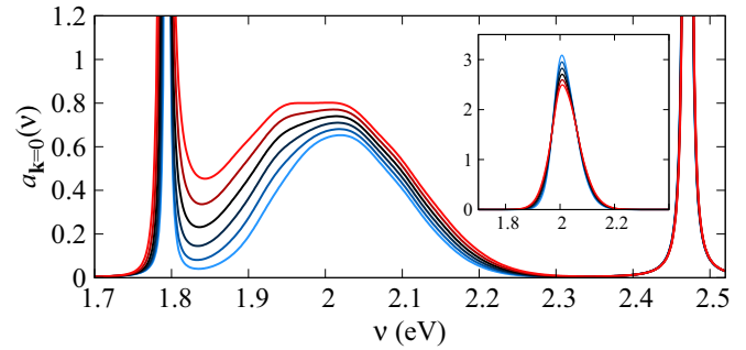
FIG. 5. Temperature dependence of absorption spectrum for a system with strong disorder \sigma = 0.025 eV. The main panel shows the optical spectrum of the strongly coupled system; the inset shows the spectrum of the bare excitons. In this case, we include two vibrational modes: S_1 = 0.2 , \Omega_1 = 0.05 eV, and S_2 = 0.3 , \Omega_2 = 0.04 eV. The height of the absorption spectra increases with increasing T in the main panel; the opposite occurs in the inset. Other parameters as in Fig. 4.
