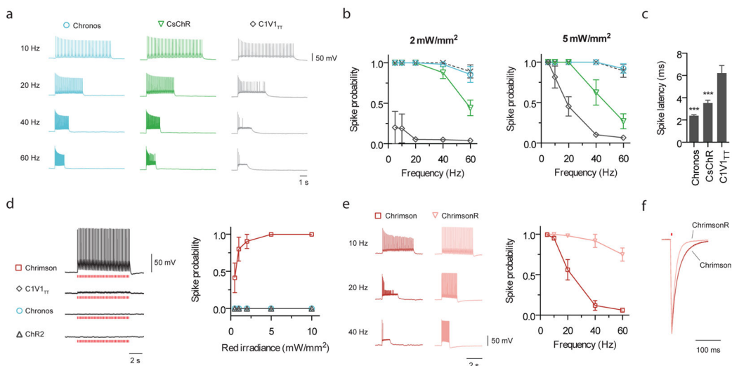
Figure 2. Comparison of optical spiking in cultured neurons (a–c) Side-by-side comparison of green light-driven spiking fidelity. All green light spiking protocols used a train of 40 pulses, 2 ms pulse width, at 530 nm, and at the indicated powers ( n = 5 - 8 cells for each opsin). (a) Representative green light driven spiking traces at the indicated frequencies at 5 mW/mm 2 . (b) Green light driven spike probability over a range of frequencies. Dashed line in b is the electrical spiking control from Chronos-expressing neurons (electrical control consisted of a train of 40 pulses at the indicated frequencies; each current injection pulse was 5 ms long and was varied from 200 – 800 pA depending on each neuron’s spike threshold). (c) Spike latencies calculated for 5 Hz trains at 5 mW/mm 2 (latency is defined as the time between light pulse onset to the spike peak). (d–f) Comparison of red light (625 nm) spiking. (d) Representative current-clamp traces of red light response and spike fidelity ( n = 5 - 8 cells for each opsin; 5 ms pulses, 5 Hz, 5 mW/mm 2 ). (e) Comparison of wildtype Chrimson and Chrimson K176R mutant (a.k.a. ChrimsonR) high frequency red light spiking ( n = 10 cells for Chrimson, n = 4 cells for ChrimsonR; 40 pulse train, 2 ms pulse width, 5 mW/mm 2 ). (f) Representative off-kinetics traces for Chrimson vs. ChrimsonR. Statistics for panel c : * P < 0.05 , ** P < 0.01 and *** P < 0.001 ; ANOVA with Dunnett’s post hoc test with C1V1TT.
