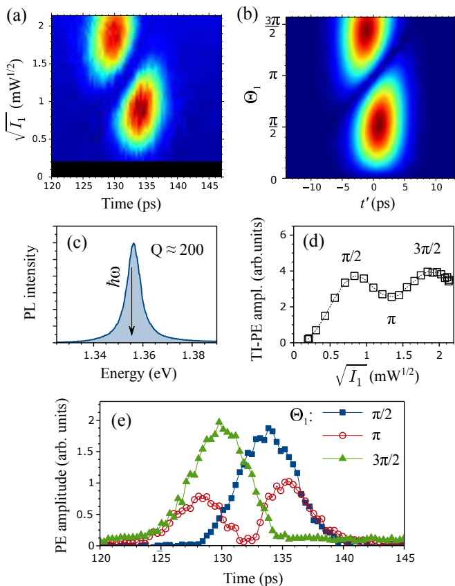
FIG. 1: (Color online) Experimental data and theoretical calculations of the absolute value of PE amplitude. (a) Experimental dependence of the PE temporal profile on the first pulse amplitude \sqrt{I_1} . (b) Theoretical modeling of the data from (a) using Eq. (2) with the following parameters: pump duration \tau_p = 2.9 ps, inhomogeneity 2\sqrt{2}\ln 2\hbar\delta \approx 0.65 meV, and rephasing pulse area \Omega_2\tau_p = \pi . In the colormaps, dark-blue indicates the zero level, dark-red corresponds to maximum signal. (c) PL spectrum of the sample with the energy position of excitation, \hbar\omega , indicated by the arrow. (d) Time-integrated (TI) modulus of the PE amplitude measured as function of the first pulse amplitude. (e) PE transients for \Theta_1 = \pi/2, \pi and 3\pi/2 , respectively.
