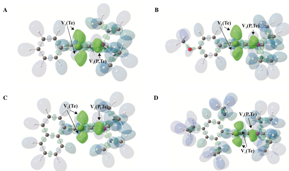
Figure S2. Isosurface representation of the localization domains of the ELL-D ( Y = 1.40 ) of 1 (A), 2 (B), 3 (C) and 5 (D), the disynaptic basins V_2(\text{Te},\text{P}) as well as the lone-pair basins ( V_1 ) of Te are colored green. All remaining ELL-D basins are given in transparent mode for clarity reasons.
