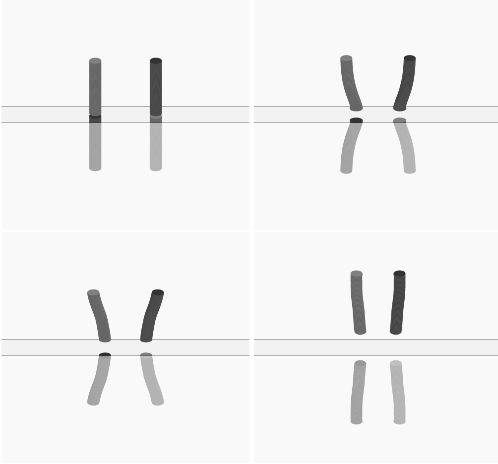
FIGURE 26. Flow evolution for anti-symmetric finite core hetons with g = 0.1 , d_y = 0.1 , and \ell_z = 0.1 , at t = 0, 10, 15 and 40 .
