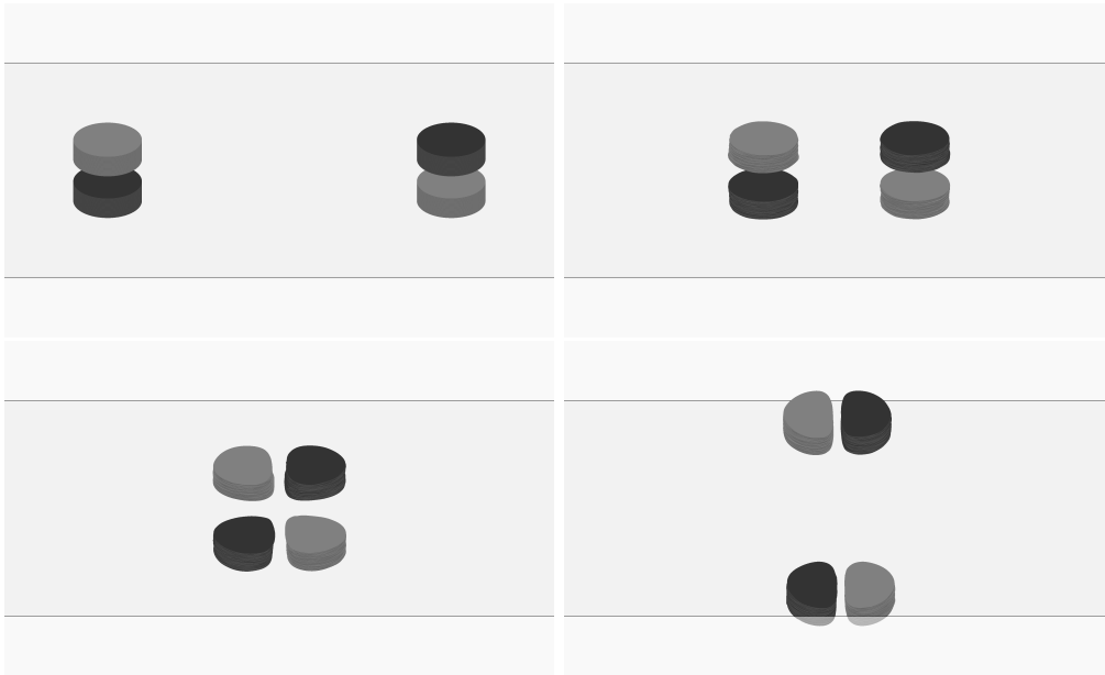
FIGURE 19. Flow evolution for anti-symmetric finite core hetons with \varrho = 1.5 , d_y = 0.1 , and \ell_z = 1 at t = 0, t = 95, 110 , and 120 . Hetons interact and poles escape as dipoles (label \square , in table 2).
