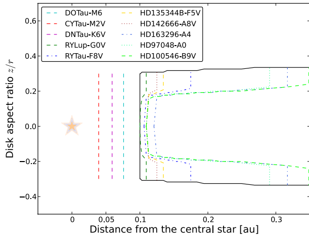
Fig. 4. Rockline position for the disks around different central stars. The thick black line indicates the disk contour at the gas density of 5 \times 10^3 \text{ cm}^{-3} for all our disk models, and we consider it as delimitation of our disk, because the erosion happens at more than 4 disk scale heights. The different colour and line styles delimit the contours of the disk with T_{\text{dust}} = 1500 \text{ K} assumed as sublimation temperature of silicates. Upward and inward of this contour, the dust is sublimated, and the disk is truncated. It describes the effective extension of the disk according to the dust sublimation temperature. For late type stars, disk temperatures are too low, and the contour is replaced by a vertical line that indicates the distance from which the dust in thermal equilibrium should be photoevaporated. The position of the central star is indicated by the star symbol.
