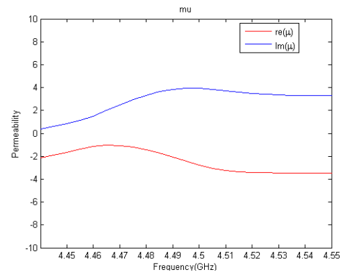
Fig. 4. The negative permeability at the desired resonant frequency (4.5GHz)
