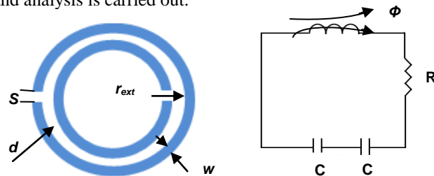
Fig. 1. Schematic of the double ring circular SSRR and its equivalent circuit
