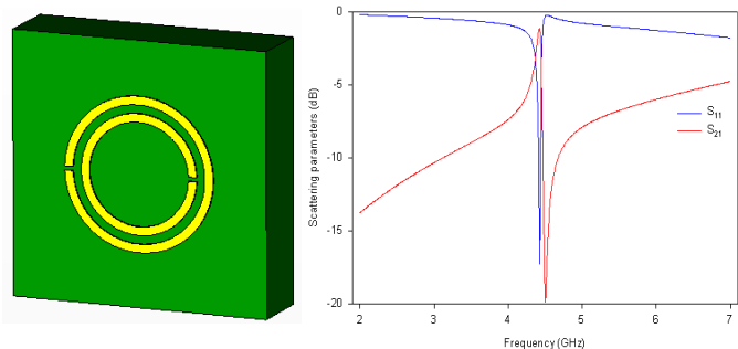
Fig. 2. The designed double ring CSRR and corresponding scattering parameters
