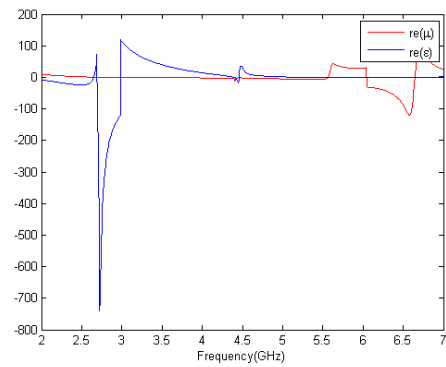
Fig. 3. The extracted permittivity and permeability of the designed CSRR
