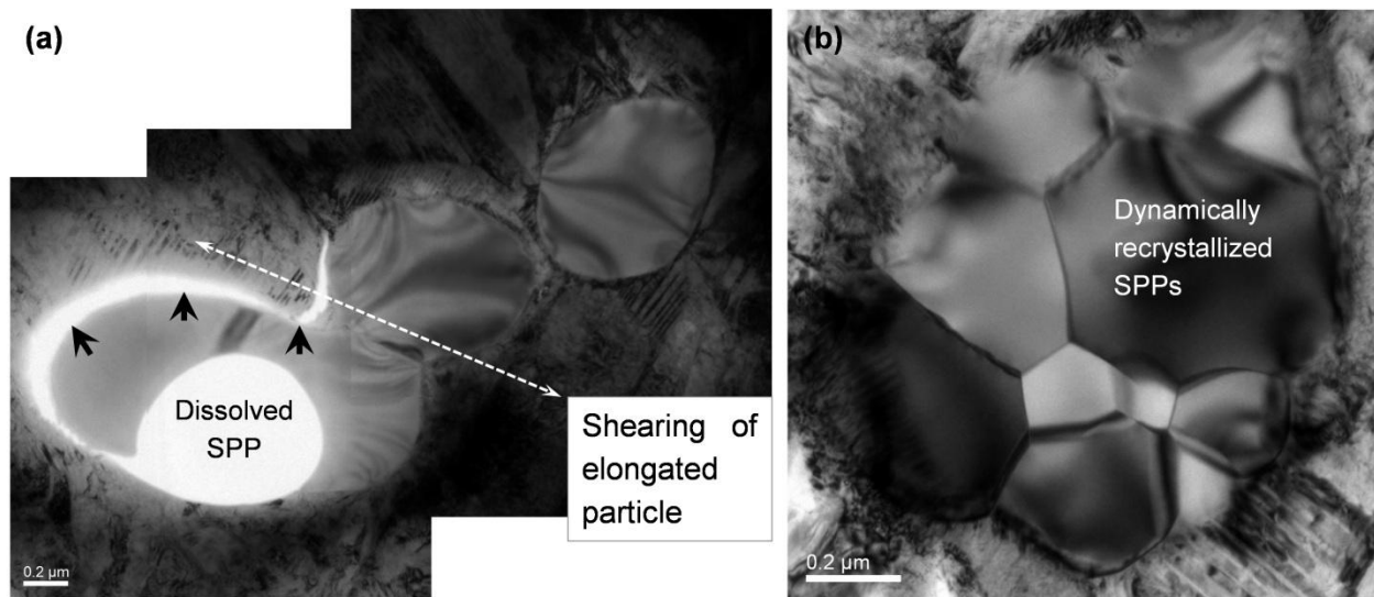
Figure 6 Microstructure of hot deformed sample after 70% reduction in cross-section (HR70) showing the deformation behaviour of Ti_2Ni SPP: (a) Necking and shearing of an elongated particle; and (b) ASPP experienced severe plastic deformation and dynamically recrystallized during hot rolling.
