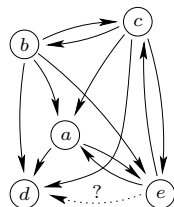
Fig. 2.1. Example 1: Associated crisp digraph and undetermined arc
