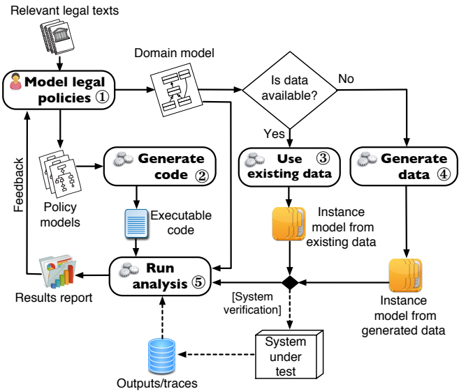
Fig. 1. Model-based Framework for Analyzing Legal Policies
