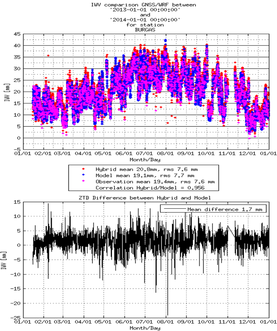
Figure 3: Top figure presents comparison of IwV computations between Hybrid in red, Model in blue and Observation in magenta. The correlation between Hybrid and Model IwVs is 0.956. The bottom figure shows the offset of the Hybrid dataset compared to the Model
