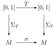
Fig. 2.2. The transformations T and \sigma .
