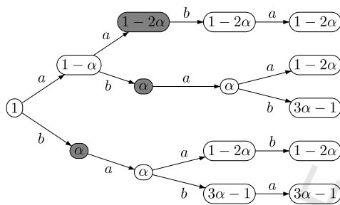
Fig. 3.1. The invariant probability distribution on the Fibonacci set.
