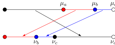
Fig. 2.1. A 3-interval exchange transformation.
