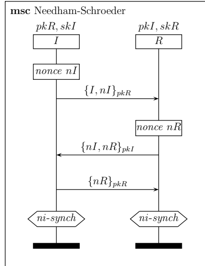
Fig. 1. The NS protocol
