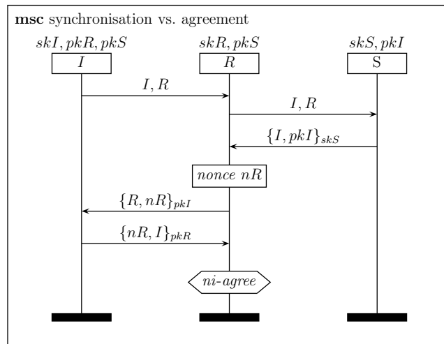
Fig. 6. A protocol satisfying NI-AGREE but not NI-SYNCH .
