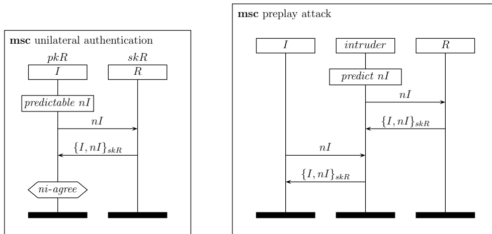
Fig. 4. Preplay attack due to a predictable nonce.
