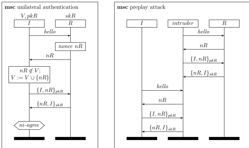
Fig. 5. Preplay attack because the nonce is controlled by the responder.
