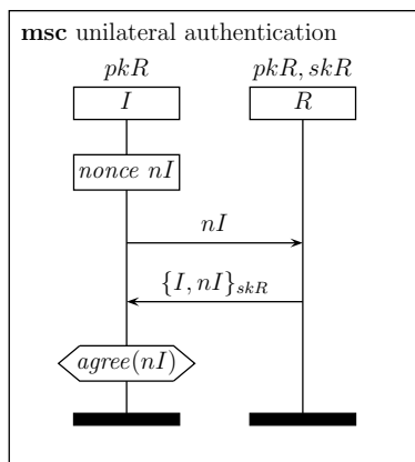
Fig. 8. Fixing the injectivity problem.
