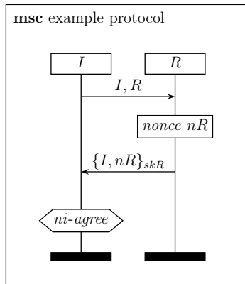
Fig. 9. A unilateral agreement protocol, with LOOP , but not injective.
