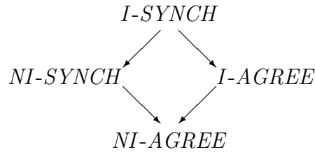
Fig. 2. Hierarchy of security properties.
