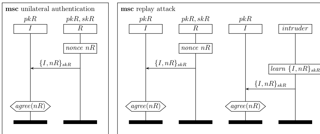
Fig. 7. An authentication protocol that is vulnerable to a replay attack.
