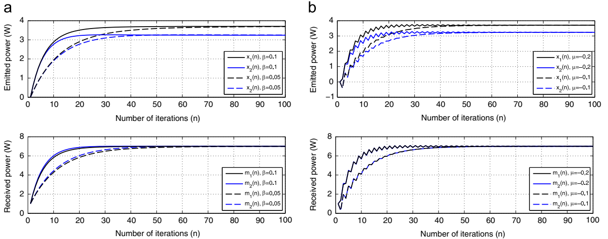
Fig. 9. Emitted and received power evolution for a 5-user asymmetric network: (a) DPC-TAS, and (b) Pricing-TAS.
