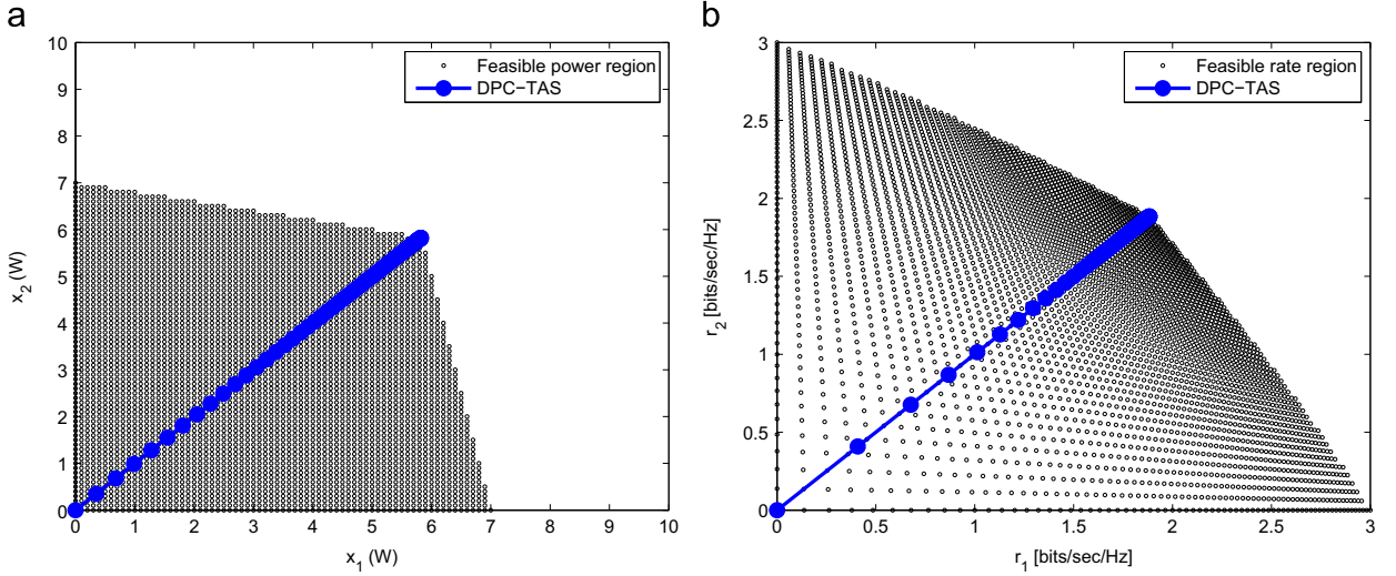
Fig. 4. Convergence of the proposed DPC-TAS for the example in Fig. 3 for \beta_k = 0.05 \forall k . (a) Power feasible set and convergence of the DPC-TAS, and (b) rate feasible set and convergence of the DPC-TAS.
