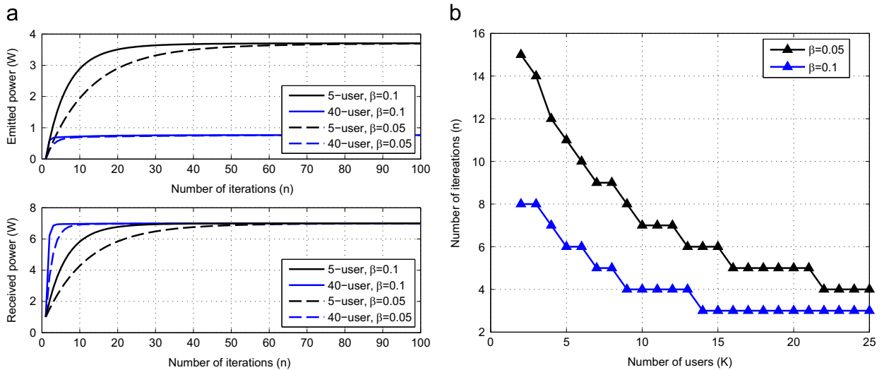
Fig. 11. Effect of network size in DPC-TAS: (a) Emitted and received power evolution of a 40-user network compared with a 5-user network, and (b) convergence time constant in number of iterations with respect to the network size.
