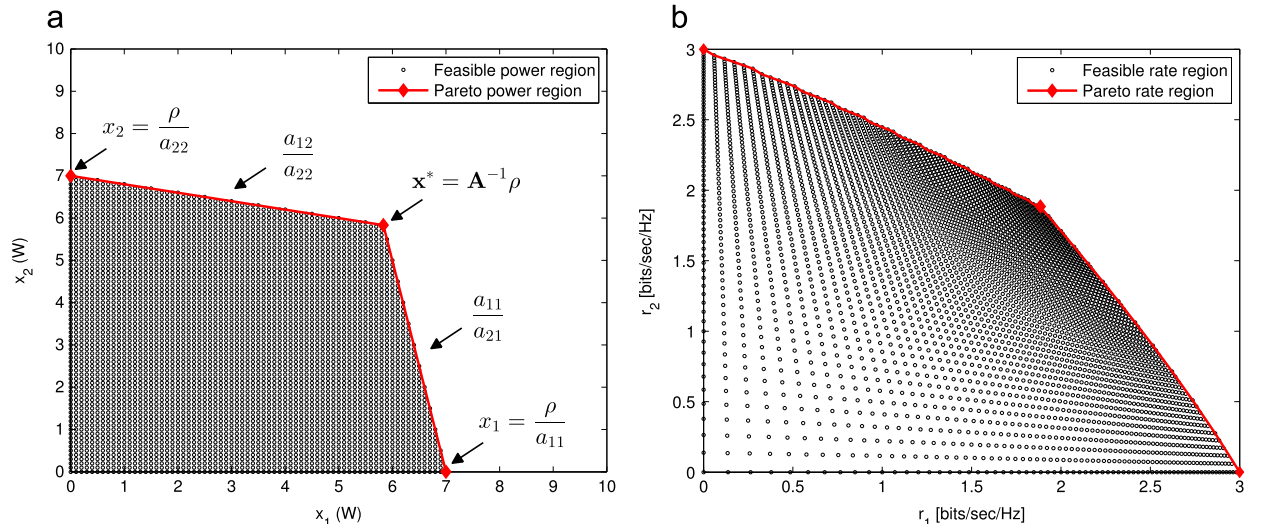
Fig. 3. Interference network with two users where \mathbf{A} = \begin{bmatrix} 1 & 0.2 \\ 0.2 & 1 \end{bmatrix} , \rho = \begin{bmatrix} 7 \\ 7 \end{bmatrix} , \mathbf{p} = \begin{bmatrix} 10 \\ 10 \end{bmatrix} . (a) TAS power Pareto and feasible set, and (b) the corresponding Pareto rate region.
