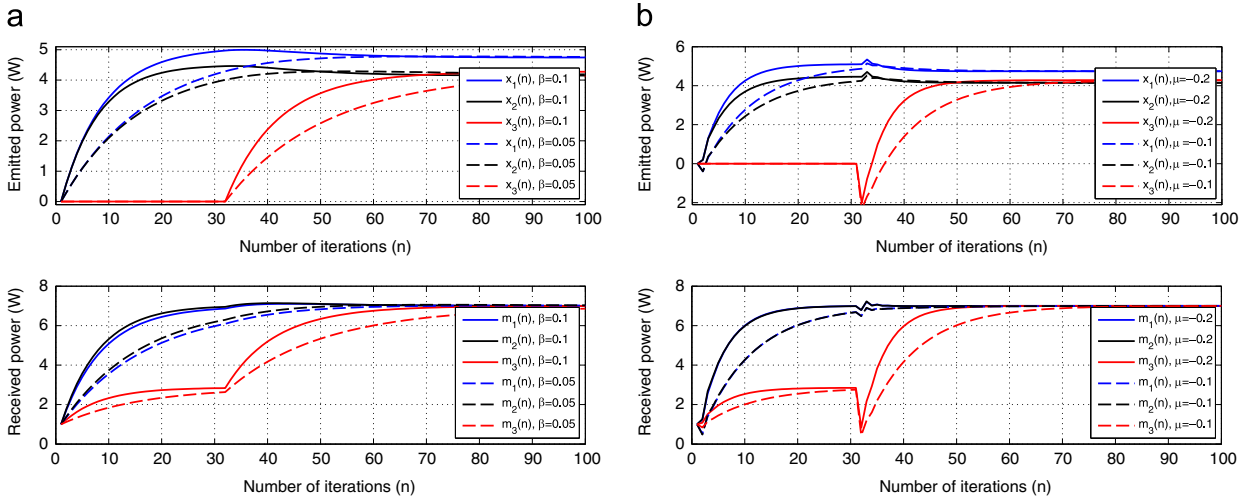
Fig. 7. Emitted and received power evolution for a 3-user asymmetric network: (a) DPC-TAS, and (b) Pricing-TAS.
