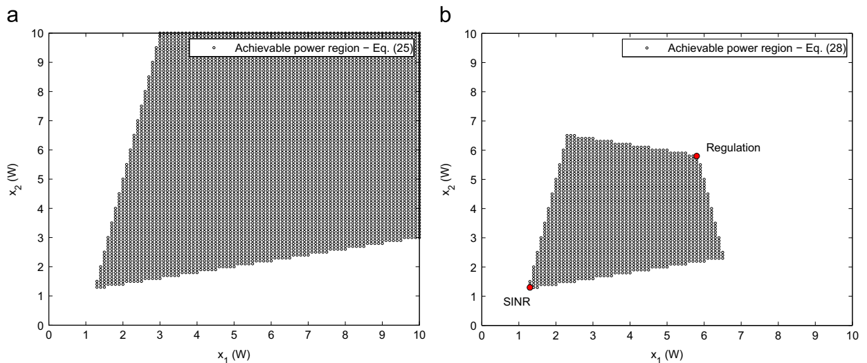
Fig. 5. Minimum QoS guarantee and DPC-TAS for the example in Fig. 3 for \gamma = \begin{bmatrix} 1 \\ 1 \end{bmatrix} . (a) SINR constraint set, and (b) Intersection of regulation and SINR sets. Red points indicate the two vertices that meet with equality either the regulation or the SINR constraints. (For interpretation of the references to color in this figure caption, the reader is referred to the web version of this paper.)
