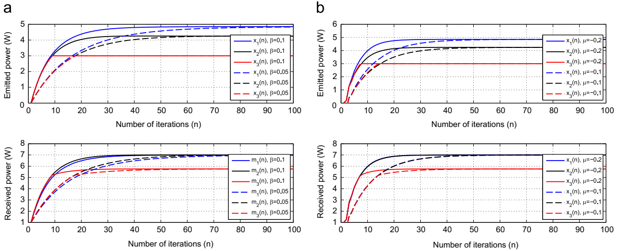
Fig. 8. Emitted and received power evolution for a 3-user asymmetric network with \mathbf{p} = [10 \ 10 \ 3]^T : (a) DPC-TAS, and (b) Pricing-TAS.
