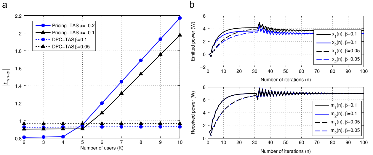
Fig. 10. Instability of Pricing-TAS: (a) Comparison of the maximum eigenvalue of the matrix (\mathbf{I} - \beta \mathbf{DA}) for DPC-TAS and the matrix \mathbf{B} for Pricing-TAS, and (b) Pricing-TAS emitted and received power evolution when number of users increases from 4 to 5.
