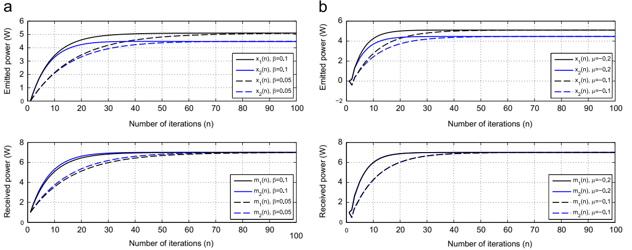
Fig. 6. Emitted and received power evolution for a 2-user asymmetric network: (a) DPC-TAS, and (b) Pricing-TAS.
